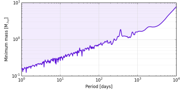
Fig. 3. Mean mass limit detection of a third body on a circular orbit as a function of period, based on current radial velocity data residuals of CoRoT-20, after removing the two identified companions. We exclude the presence of any companions in circular orbits in the light-blue region.
