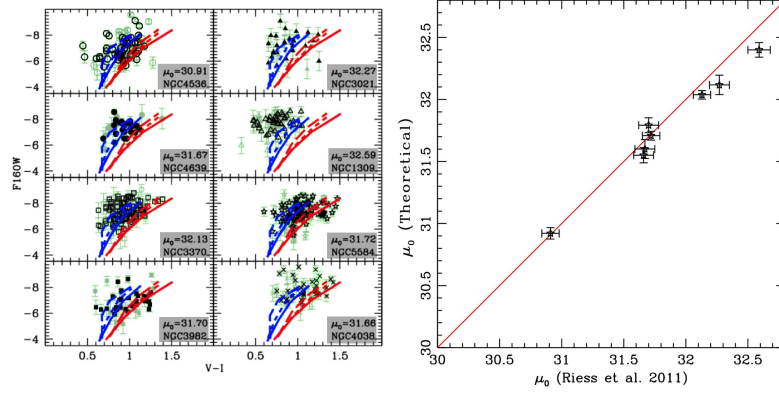
Fig. 2 Left: As in Fig. 1 (right panel) for all the other CC samples. In this case, dark and light green symbols represent good and rejected CCs (see [17] for details), respectively. Right: the comparison between the distance moduli obtained using our theoretical F160W PL for Z = 0.02 Y = 0.28 and for periods larger than 10 d and those obtained by [17]
