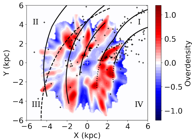
Fig. 5. Comparison between the measured overdensity map presented in this work (Figure 1B), the distribution of the maser sources (black crosses) and spiral arm model (solid lines, from left to right: Outer, Perseus, Local, Sagittarius-Carina, Scutum arm) from Reid et al. (2019), and the Perseus arm from Levine et al. (2006) (dashed line). Roman numerals show the I, II, III and IV Galactic quadrants.
