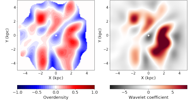
Fig. B.2. Same as Figure 1B (left panel) and C (right panel), but using a larger scale length h = 0.8 kpc, which corresponds to scale=4 of the wavelet transform.
