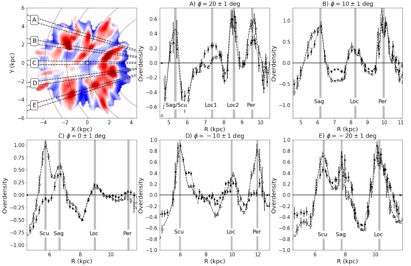
Fig. 2. Top left panel: Same as Figure 1B, but with some geometric references superimposed. Dotted lines from left to right show the points with constant Galactocentric radius R=12, 10, 8, 6 kpc, respectively. Dashed lines show the five selected slices (A,B,C,D,E), which are separated by 10 deg in Galactic azimuth \phi and of 2 deg in width. Panels A to E: The profile of the measured overdensity as a function of R for the UMS P18 sample (black dots) and the Z21 sample (white squares). Error bars show bootstrap uncertainties, calculated as explained in Appendix B.3. For computational reasons, black dots/white squares and relative errorbars were calculated for each slice and then connected using splines, as shown by the dotted (dashed) lines, to give a visual impression of how the overdensity varies at different radii. Each peak of the measured overdensity has been identified with a spiral arm in the Milky Way, as indicated by the vertical grey lines and the corresponding labels. The identification of each peak is not due to an assumed specific model, but is simply based on the geometric appearance of the top left panel (see text).
