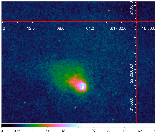
Figure 1. X-ray image from the merged, 152 ks duration, Chandra -ACIS observation restricted to the 1.0–5.0 keV energy range and covering a 4'.75 \times 3'.75 region near the aimpoint and smoothed using a Gaussian kernel of 3 pixel ( 1''.48 ) radius. Colors are proportional to the number of X-ray events per pixel using a square root scaling. CXOU J061705.3+222127 is the bright white object surrounded by a ring (light blue) and the comet-shaped PWN (red and green). Relatively low surface brightness structure (dark blue to black) is visible throughout the S3 field of view. The center of the IC 443 supernova remnant lies \sim 30' to the N of J0617.
