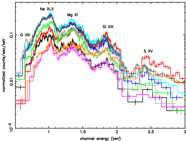
Figure 9. Observed spectra of the nine numbered regions shown Figure 8. The spectra have been binned up to 10 channels in order to achieve a minimum detection significance of 10 for display purposes. Colors correspond to regions 1: cyan, 2: gray, 3: magenta, 4: blue, 5: black, 6: green, 7: red, 8: orange, 9: dark gray as defined in Figure 8 and Table 1. Note the high flux above \sim 2.0 keV in the spectrum of regions 7–9 indicating a strong hard spectral component. The different relative strengths of emission lines among the various regions are due, in part, to real differences in elemental abundances as the best-fitting models all have similar plasma temperatures and absorption columns (Table 1).
