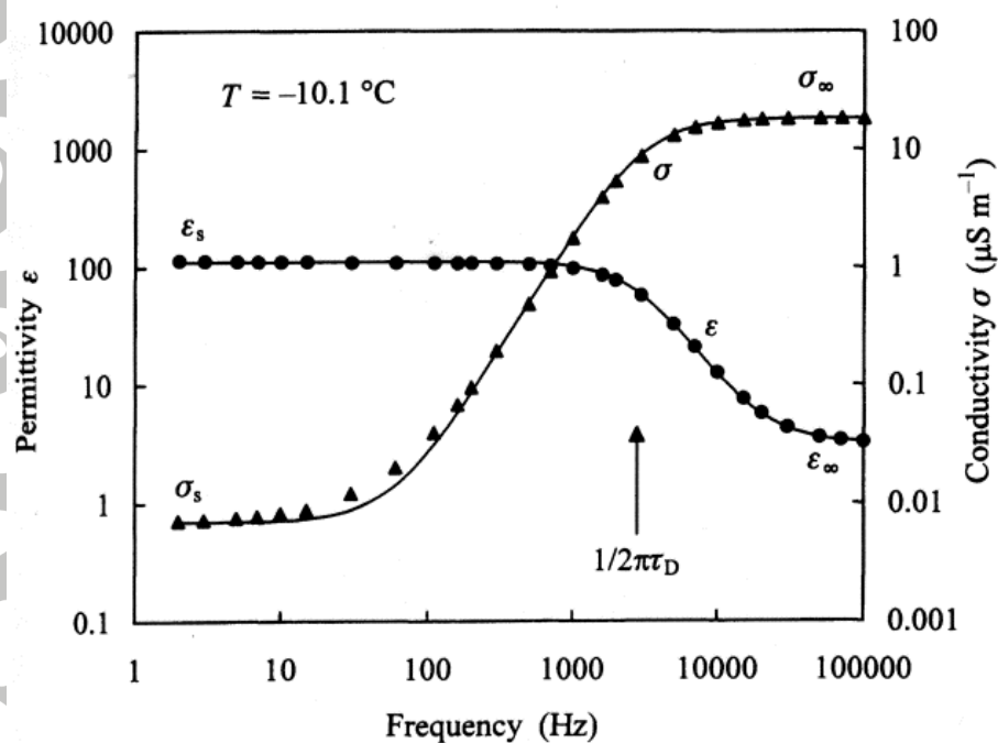
Figure 9 Real part of permittivity and conductivity as a function of frequency (2 Hz-100 kHz) of a single crystal of pure water ice measured at 263 K (Takei and Maeno [1997] modified by Petrenko and Whitworth [1999]).
