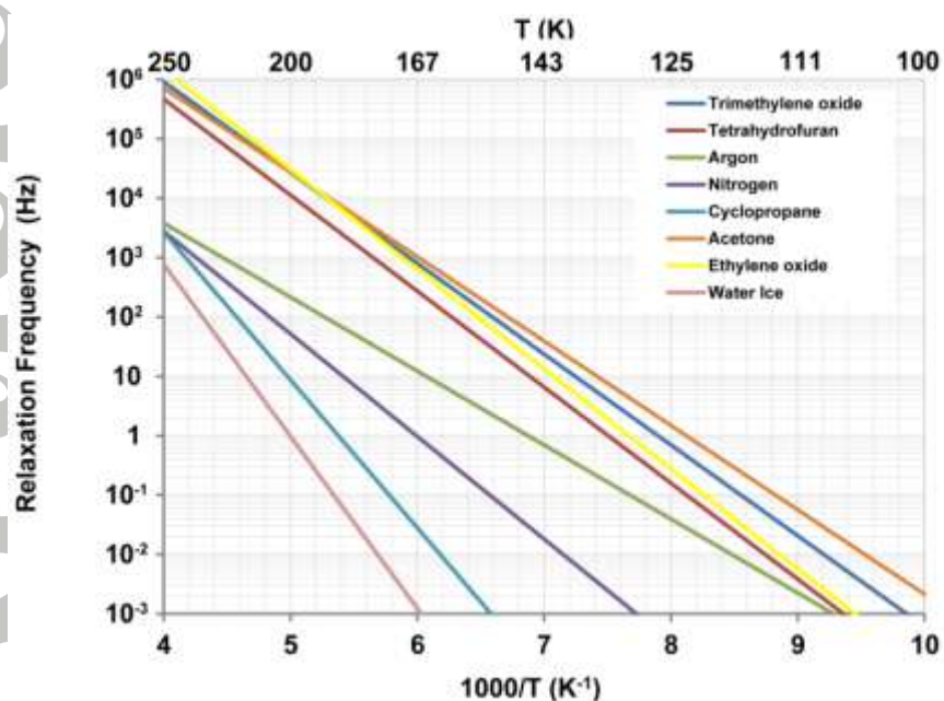
Figure 14 Relaxation frequencies of some clathrate hydrates and pure water ice as a function of temperature, extrapolated from Table 6. The comparison of the various curves shows that the relaxation frequencies of these compounds are always higher than that of pure water ice and that such differences increase with decreasing temperatures. The legend indicates the guest molecules (cf. Table 6).
