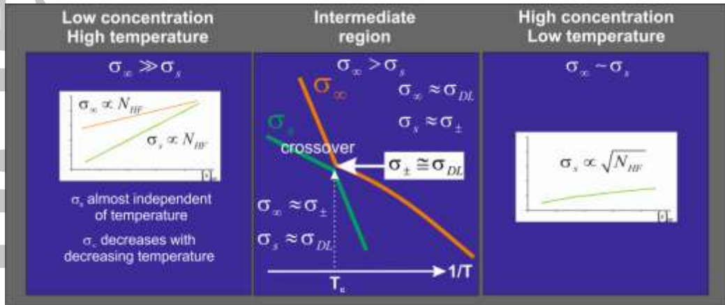
Figure 11 Summary of the dielectric properties of HF doped ice for different concentrations and temperature ranges. The orange curve refers to \sigma_\infty and the green curve to \sigma_s . In the low concentration and high temperature range (left panel) the high frequency conductivity is much larger than the static conductivity; in the intermediate region (central panel) \sigma_\infty is still larger than \sigma_s , except at the crossover temperature, where \epsilon_s - \epsilon_\infty = 0 ( \sigma_{DL} \cong \sigma_\pm ), and the ice behaves as a pure conductor. In the high concentration and low temperature regime (right panel) the high and low frequency conductivity are of the same order of magnitude and the trend of \sigma_s vs concentration becomes non-linear.
