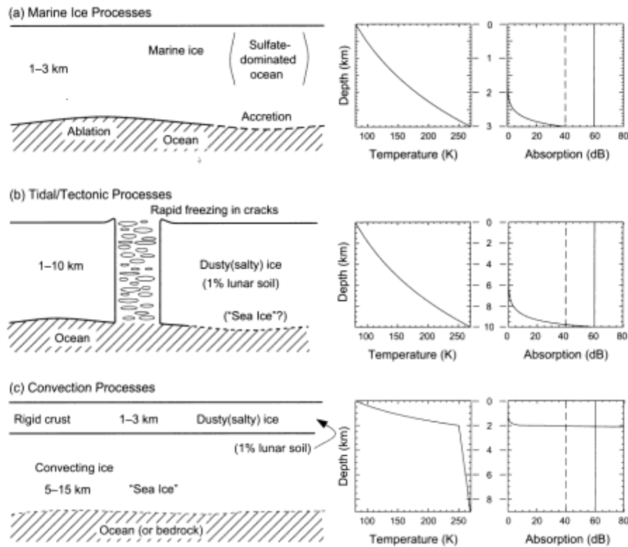
Figure 18 Europa icy crust models proposed by Moore [2000] (left) and relevant radar signal absorption vs. depth (right) [taken from Blankenship et al. , 2009]. a) Conductive ice shell similar to terrestrial marine ice; b) icy crust subjected to tectonic process with extrusions of molten material; c) convective ice shell below a thin rigid stagnant lid. Dashed and solid lines in right panels represent the expected signal to noise ratio for the jovian and anti-jovian sides.
