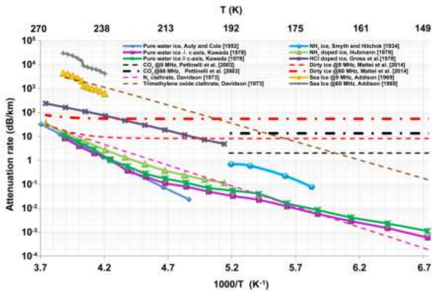
Figure 17 Attenuation rate vs. 1/T estimated at 9 MHz and 60 MHz for different types of ice using Equation 6 and the data available in the literature. If not specifically indicated in the legend, the curves at 9 MHz and 60 MHz coincide.
