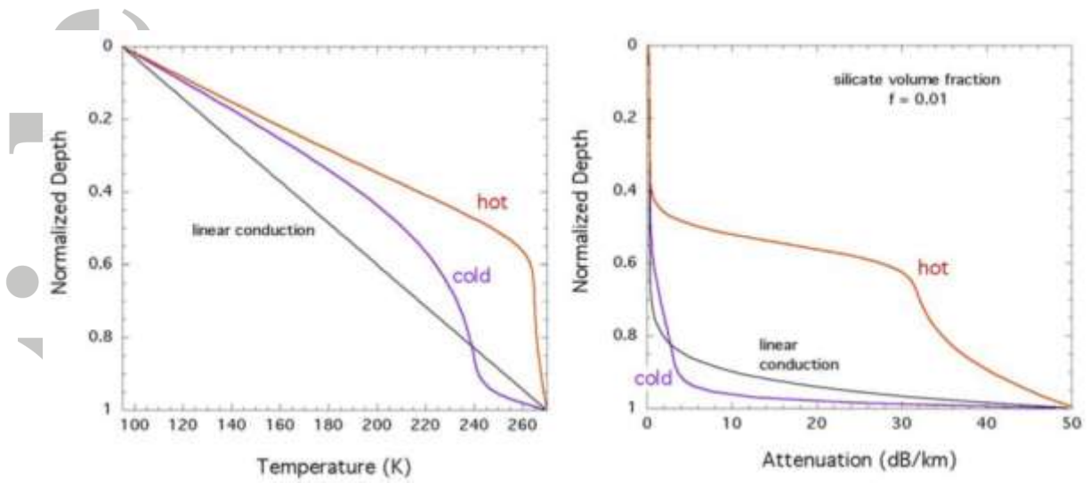
Figure 19 Thermal profiles (left) and radar signal attenuation at 50 MHz (right) in the cold/hot convective plumes for the european crust (taken from McKinnon [2005]).
