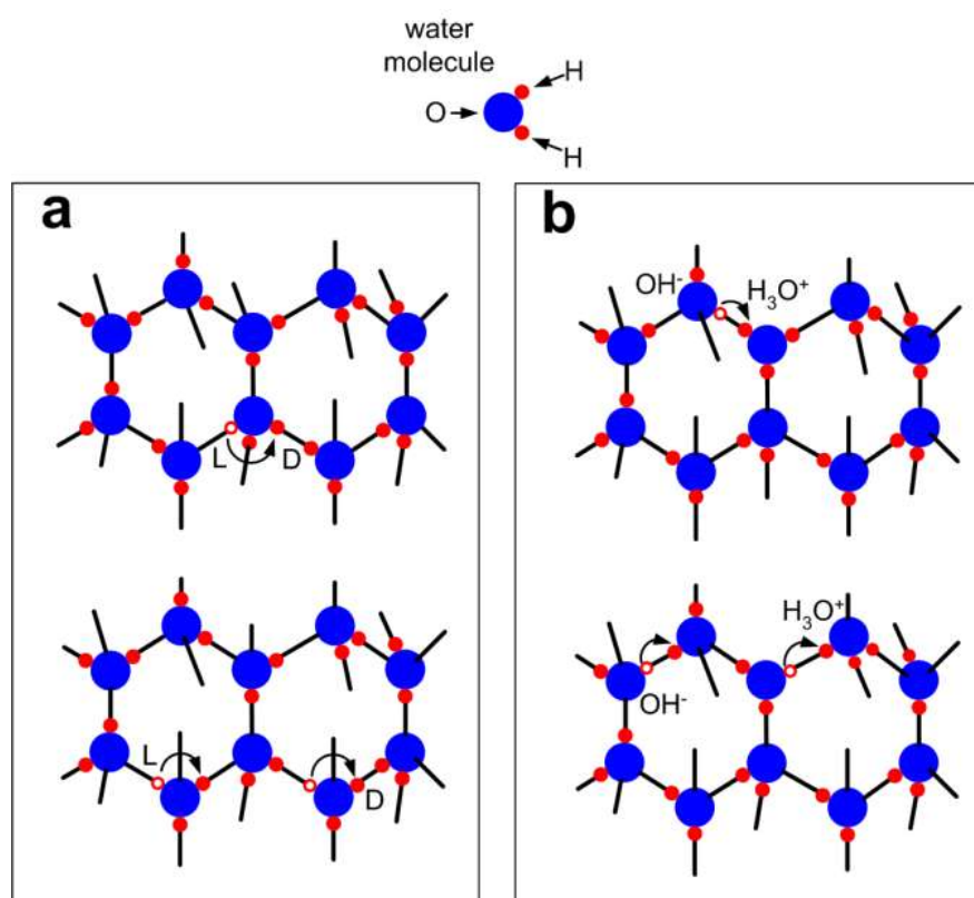
Figure 8 Intrinsic defects and associated protonic motions for L-D defects (a) and ionic defects (b).
