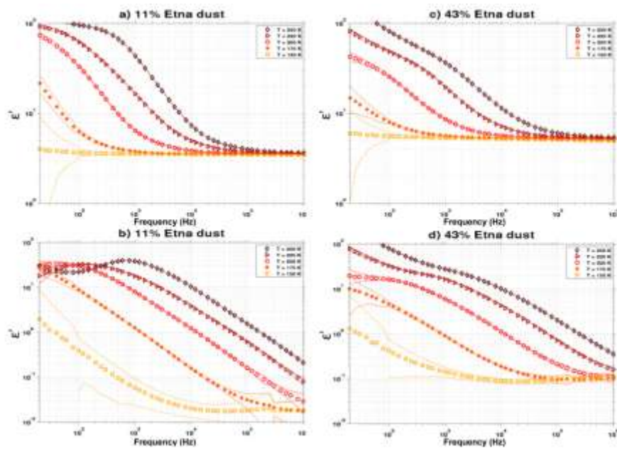
Figure 16 Electromagnetic properties measured on two ice/grains mixtures at different temperatures. Panels a and c show the real part of permittivity and panels b and d the imaginary part of permittivity. The dashed lines represent the data uncertainties indicating the envelope of the error bars. Note that they are only visible if larger than 1% (modified from Mattei et al. 2014).
