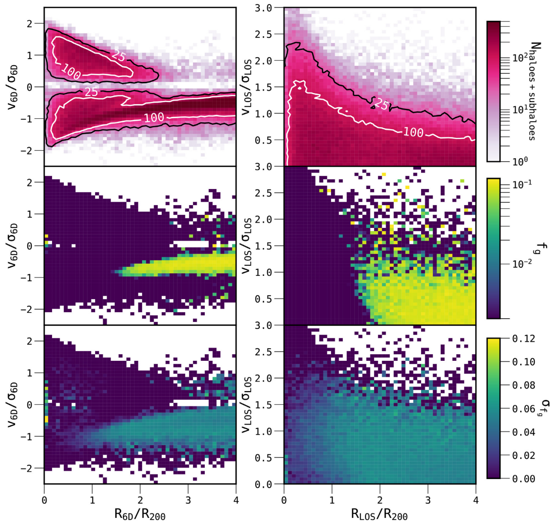
Figure 5. The stacked phase-space plane for all 324 clusters in THE300 project. Both haloes and subhaloes are included in all panels. The left- and right-hand columns are in 6D and LOS perspectives, respectively. The planes are stacked on a 50 \times 50 grid where the top row shows the number of haloes and subhaloes in each bin, the middle row indicates the median gas fraction in each bin, and the bottom row illustrates the gas fraction standard deviation in each bin. Contours are included in the top row, indicating the number of haloes and subhaloes encapsulated in each. The 6D perspective shows two distinct infalling and outgoing populations of objects, which are not seen in the LOS perspective. Also, from the 6D perspective, first infallers are substantially more gas-poor and appear to lose their gas at \sim 1.5R_{200} , whereas the cut-off in gas-rich objects in the LOS perspective occurs closer to \sim 2R_{200} .
