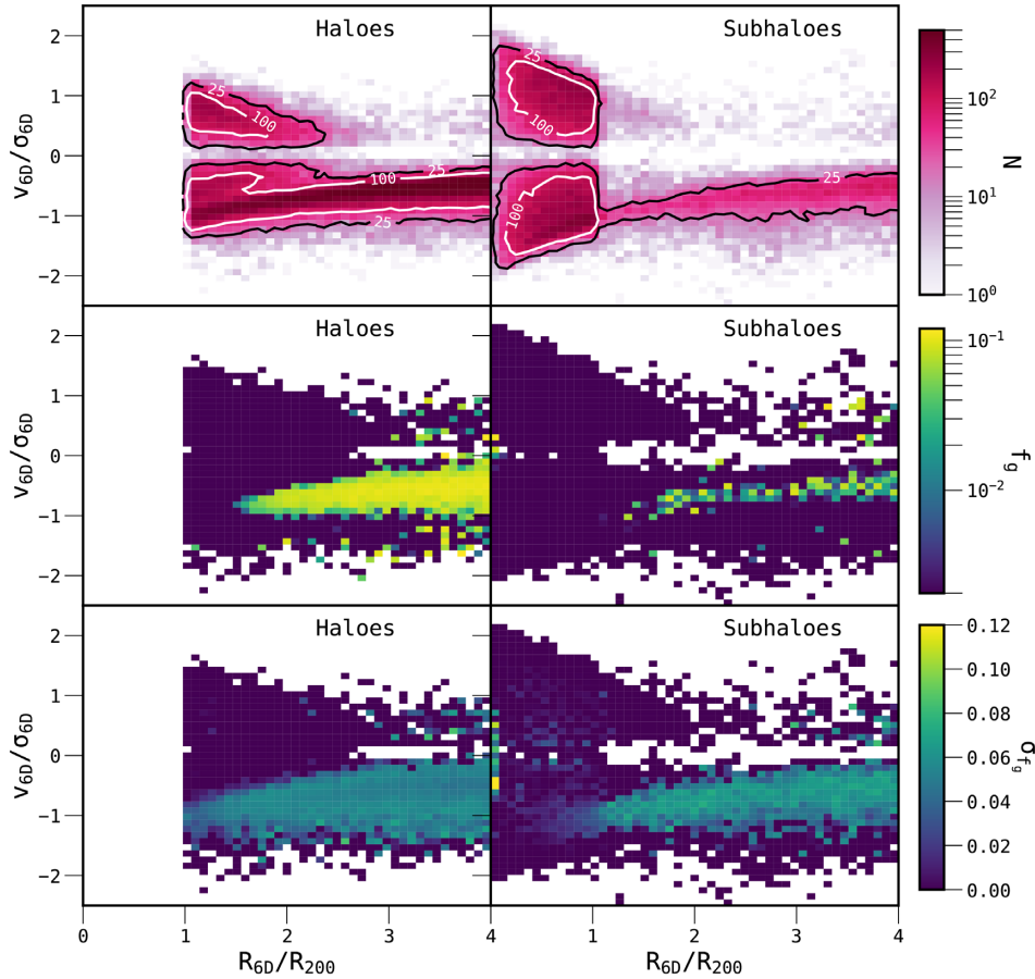
Figure 7. The stacked phase-space planes for all 324 clusters in THETHREEHUNDRED project, split by subhalo status. The left- and right-hand columns show only haloes and subhaloes respectively in the 6D perspective. The planes are constructed as in Fig. 5. \sim 10 per cent of all infalling objects are in the form of subhaloes, which are substantially more gas-poor than haloes in the same phase-space location.
