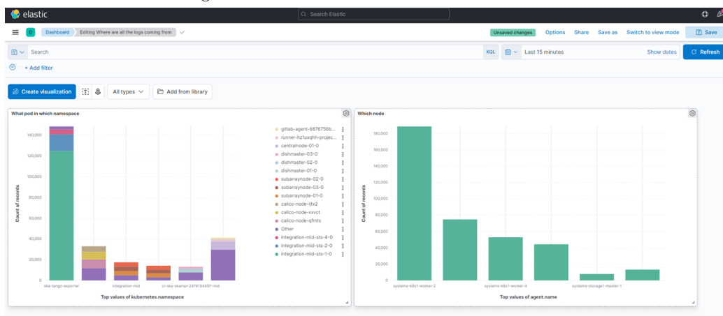
Figure 11. Kibana dashboard
