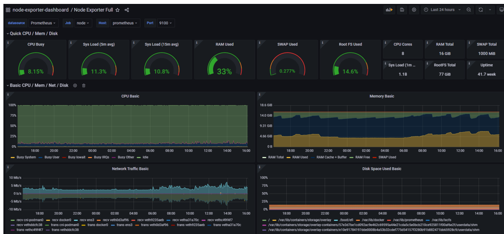
Figure 7. Node exporter dashboard
