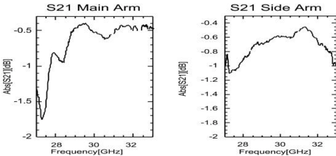
Fig. 2: OMT Insertion Loss measurements.
