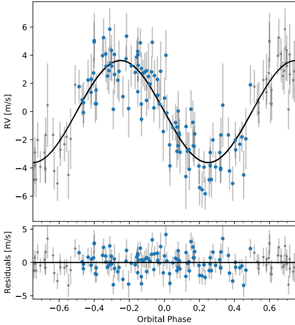
Fig. 10. Top panel: phase-folded RV fit obtained using PyORBIT. Activity jitter and long-term trend both removed. Larger blue dots delineate the RV variation over a single orbital cycle. Bottom panel: residuals from the best fit.
