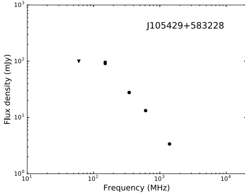
Figure 20. An example of one unusual USS source detected in the Lockman Hole. This source has an ultra steep spectrum of \alpha_{150}^{400} = -1.6 between 150 and 1.4 GHz, but is undetected at 60 MHz and therefore has a much flatter spectral index from 60–150 MHz of \alpha_{60}^{150} > -0.07 (assuming a 5\sigma upper limit at 60 MHz).
