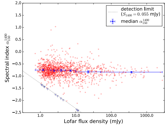
Figure 16. Median spectral index as a function of 150 MHz flux density for sources in the Lockman–WSRT sample. The small red points show the individual measurements for all sources in the sample while the blue squares show the median spectral index in each bin (these are shown in Table 5). The horizontal error bars denote the bin widths and the vertical errorbars represent the 95 per cent confidence interval of the median (from bootstrap). Blue triangles mark the upper limits of the spectral index for sources detected in the LOFAR catalogue that do not have a WSRT counterpart (see Section 5.2.1).
