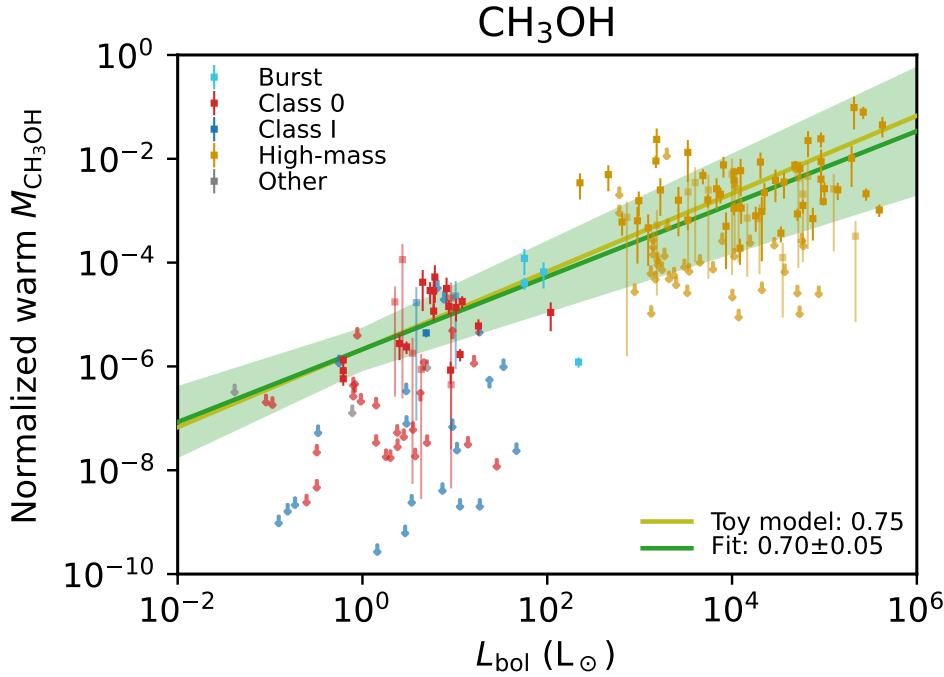
Fig. 4. Normalized warm gaseous \text{CH}_3\text{OH} mass, M_{\text{CH}_3\text{OH}}/M_{\text{dust},0} , as a function of the bolometric luminosity. Different colors denote different observational classes, and all sources with L_{\text{bol}} > 1000 L_{\odot} are classified as high-mass sources. Additionally, sources that are suggested to currently be in a burst phase (e.g., V883 Ori and IRAS2A; van 't Hoff et al. 2018; Lee et al. 2019b; Hsieh et al. 2019) are highlighted. Sources in the “other” category include Class II and flat spectrum sources. The green line indicates the best-fit power-law model to the data points (excluding the upper limits) and the green shaded area the 3\sigma uncertainty on the fit. The yellow line indicates the relation for the toy model of Eq. (4) scaled to match the best-fit power-law model.
