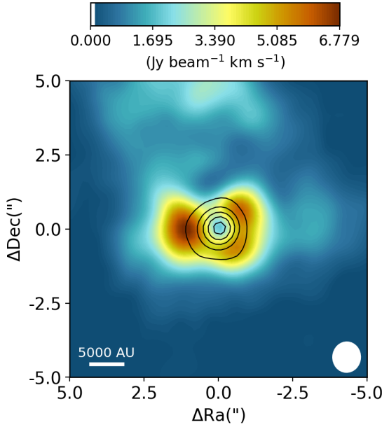
Fig. 6. Integrated intensity maps of the \text{CH}_3\text{OH} 8_{0,8}-7_{1,6} line for 693 050. The color scale is shown on top of the image. The image is integrated over [-5, 5] \text{ km s}^{-1} with respect to the V_{\text{lsr}} . The white vertical line in the colorbar indicates the 3\sigma threshold. The continuum flux is indicated with the black contours at [0.1, 0.3, 0.5, 0.7, 0.9] times the peak continuum flux, F_{\text{cont}} = 1.92 \text{ Jy beam}^{-1} . The white ellipse in the lower right of each image depicts the beam size, and in the lower left a physical scale bar is displayed.
