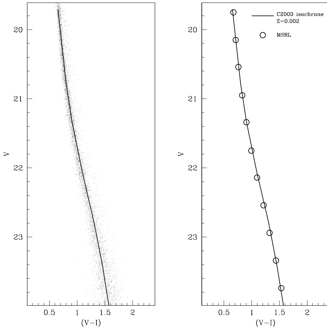
FIG. 8.—Comparisons between the Cassisi et al. (2000) isochrone adopted to convert masses to V magnitudes and the observations. In the left panel the isochrone (solid line) is superposed onto the observed CMD. In the right panel it is superposed onto the MSRL (large open circles).
