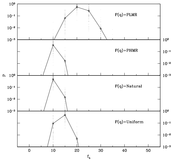
FIG. 12.—Estimates of the binary fraction in the whole observed sample (Int+Ext), for the four F(q) distributions we considered. In each panel the probability that the actual simulated sample is drawn from the same parent population as the observed sample (according to a K-S test) is plotted vs. the binary fraction introduced in the simulated samples. Each small dot represents one of the 100 random realizations of the simulated sample at a given [f_b, F(q)] pair. The open circles are the average probability of the 100 realizations of simulated samples. A line connecting the open circles has been drawn as an aid for the eye. The figure has been arranged to be as similar as possible to the corresponding plots by RB97.
