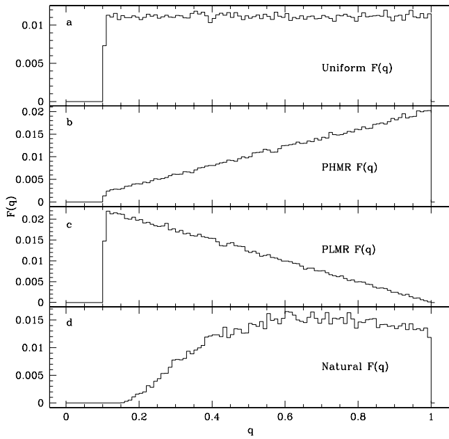
FIG. 10.—Normalized histograms of 100,000 binary systems randomly drawn from the adopted F(q) distributions. (a) Uniform distribution. (b) PHMR distribution. (c) PLMR distribution. (d) Natural distribution. The limit q > 0.1037 has been applied to all the distributions to exclude stars/brown dwarf systems from the estimate of the total binary fraction.
