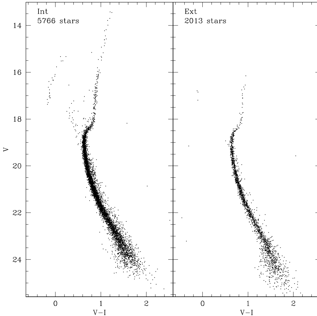
FIG. 2.— (V, I) CMDs of the Int (left panel) and Ext (right panel) fields. Only the stars with observational errors lower than 0.1 mag in each filter are presented in the plots. Stars brighter than V \sim 16.0 in the Ext field have saturated images and are not shown.
