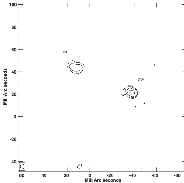
Figure 2. EVN map of the radio continuum emission in IRAS15480 at 5 GHz (Castangia et al. in prep.). Contour levels are (-1, 1, 2, 4, 8 \dots) \times 0.2 \text{ mJy/beam} ( 5\sigma ).
