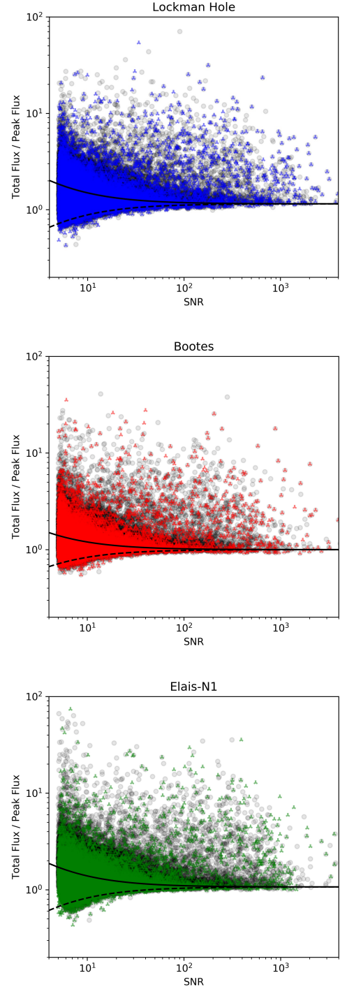
Fig. 3. Total to peak flux density ratio as a function of signal to noise ratio ( S/N = S_{\text{peak}}/\sigma ) for both the raw (black transparent circles) and final ( \Delta symbols in blue, red and green colors) catalogs in the LH, Boo and EN1 fields (respectively from top to bottom panels). The dashed and solid lines represent the unresolved source distribution lower and upper envelopes respectively (see text for more details).
