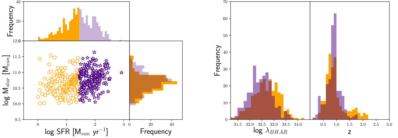
Fig. 4. SFR as a function of host galaxy stellar mass (Left Panel) for low ( \log SFR \lesssim 1.4 ) and high ( > 1.4 ) SFR subsamples. The corresponding distribution in terms of M_{star} , \lambda_{BHAR} , SFR and spectroscopic redshift (Right Panel) are shown for the two subsets
