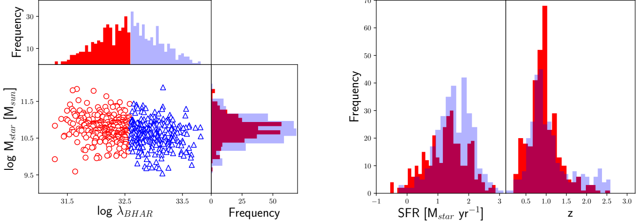
Fig. 3. Specific BHAR as a function of host galaxy stellar mass (Left Panel) for low ( \log \lambda_{BHAR} \lesssim 32.6 ) and high ( > 32.6 ) specific BHAR subsamples. The corresponding distribution in terms of M_{star} , \lambda_{BHAR} , SFR and spectroscopic redshift (Right Panel) are shown for the two AGN subsets.
