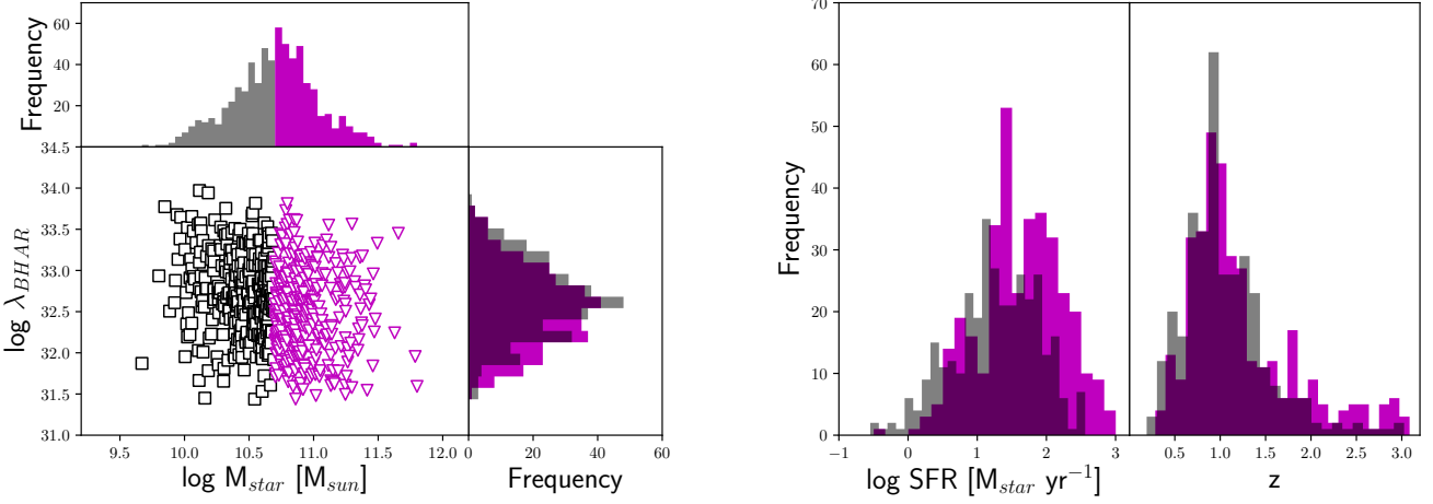
Fig. 2. Host galaxy stellar mass as a function of specific BHAR (Left Panel) for low ( \log M_{star}/[M_{\odot}] \lesssim 10.75 ) and high ( >10.75 ) stellar mass subsamples. The corresponding distribution in terms of M_{star} , \lambda_{BHAR} , SFR and spectroscopic redshift (Right Panel) are shown for the two AGN subsets.
