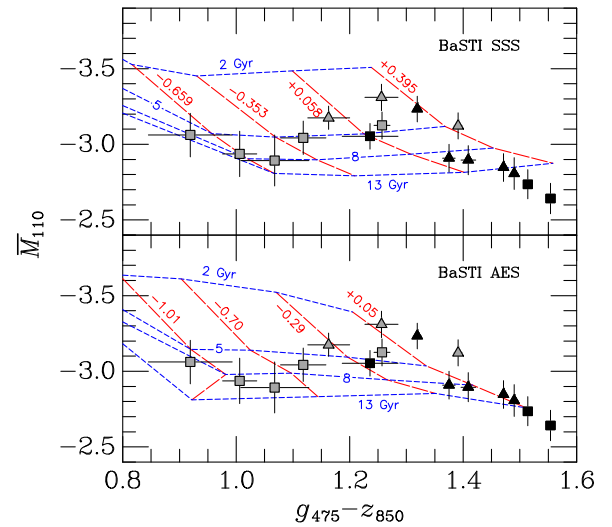
Figure 6. Teramo BaSTI models compared to \bar{M}_{110} as a function of galaxy ( g_{475}-z_{850} ) color for two metallicities variants of the models computed using the individual galaxy distances: the “SSS” models (top panel) are solar-scaled abundances spanning the range from [\text{Fe}/\text{H}] = -0.659 to +0.395 . The “AES” models (lower panel) have enhanced \alpha element compositions and reduced [\text{Fe}/\text{H}] to make the overall metallicity Z the same as the solar-scaled models shown in the top panel. The range of [\text{Fe}/\text{H}] spanned by the AES models is -1.01 to +0.05 . Lines of constant metallicity are shown with red dashed lines, and lines of constant age from 2 to 13 Gyr are plotted with dotted blue lines.
