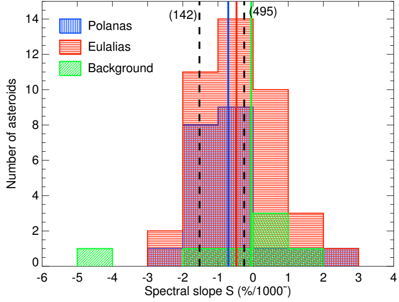
Figure 5: Distribution of the spectral slope S' for the asteroids of the Polana (blue) and Eulalia (red) families, and of the background population (green). The spectral slope has been computed between 0.55 and 0.90 \mu\text{m} . Colored vertical lines correspond to the mean slope of each group. Vertical dashed lines indicate the spectral slope of asteroids (142) Polana and (495) Eulalia.
