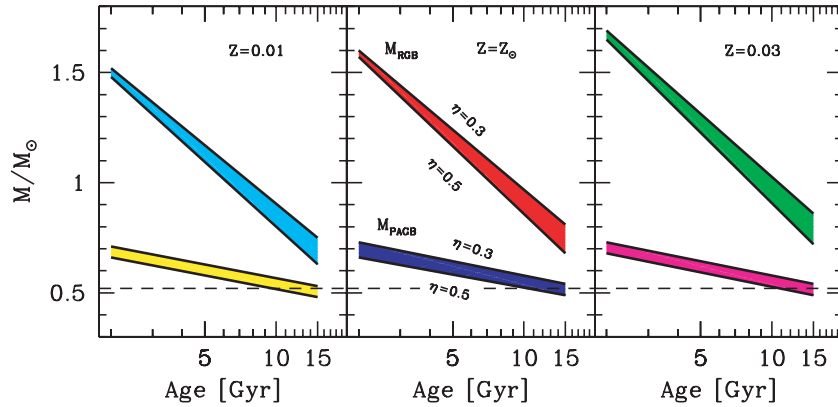
Figure 3. Time evolution of the stellar mass at some tipping points across the H–R diagram for SSPs of different metallicity Z , about the solar value, as labelled in each panel. Upper strips in each panel are the theoretical loci for stellar mass at the tip of the RGB evolution ( M_{\text{RGB}} ) according to a Reimers mass-loss parameter in the range 0.3 \leq \eta \leq 0.5 , as labelled in the middle panel, for general reference. Lower strips mark the locus for stellar mass at the onset of PAGB evolution ( M_{\text{PAGB}} ), again for the same reported range of the mass-loss parameter \eta . The minimum mass for stars to reach the AGB thermal pulsing phase (and eventually produce a PN) is marked by the dashed line, according to Dorman et al. (1993) and Blöcker (1995).
