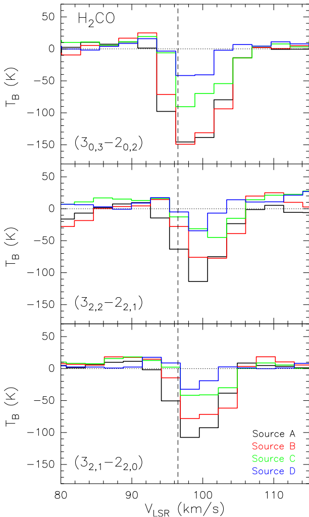
Fig. 5. Same as Fig. 3, but for H_2CO ( 3_{0,3}\text{--}2_{0,2} ) ( E_{\text{up}}/k_B = 21 \text{ K} ), ( 3_{2,2}\text{--}2_{2,1} ) ( E_{\text{up}}/k_B = 68 \text{ K} ), and ( 3_{2,1}\text{--}2_{2,0} ) ( E_{\text{up}}/k_B = 68 \text{ K} ). The x-axis is in units of velocity. The vertical dashed line indicates the systemic LSR velocity of 96.5 \pm 0.5 \text{ km s}^{-1} (Beltrán et al. 2018).
