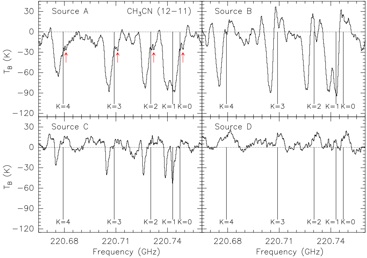
Fig. 3. \text{CH}_3\text{CN} (12–11) spectra of the K = 0, 1, 2, 3 , and 4 transitions averaged over a beam toward the position of the dust continuum emission peak of the four sources embedded in the Main core of G31. The black lines indicate the different K components shifted to the frequency of the ambient gas velocity ( 96.5 \text{ km s}^{-1} ). The red arrows in the top left panel indicate the secondary absorption component at blueshifted velocities associated with source A.
