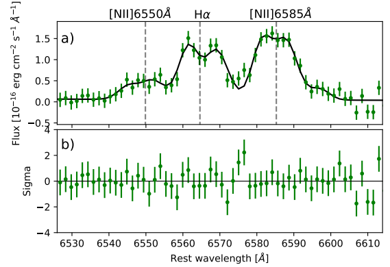
Fig. 3. Residual spectrum of SDSS J1431+4358 (green symbols in this figure and in Fig. 1) around the H\alpha + [NII] \lambda 6550 Å, \lambda 6585 Å emission line region. The spectrum is shown in the rest-frame vacuum wavelengths. The gray dashed vertical lines mark the position of the emission line at the systemic velocity of the host galaxy. Panel a: the black solid line is the model obtained by the combination of a power-law continuum plus two Gaussian emission line components for both the H\alpha and for each of the [NII] emission lines. Panel b: relevant residuals, shown in terms of sigmas.
