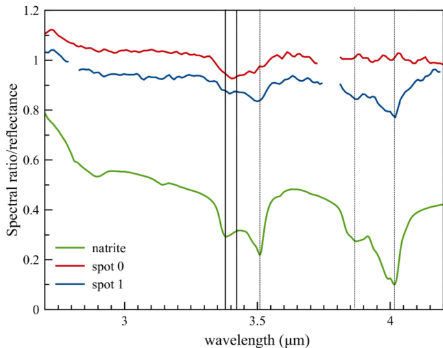
Figure 5. Spectral ratio of spot 0 and 1 with background in comparison to a laboratory spectrum of natrite CB-EAC-034-C, (RELAB). Vertical dotted lines highlight the carbonate absorption minima, and solid vertical lines indicate CH 2 (3.42 μm) and CH 3 (3.38 μm) main absorptions. The line at 3.42 μm corresponds also to a carbonate absorption.
