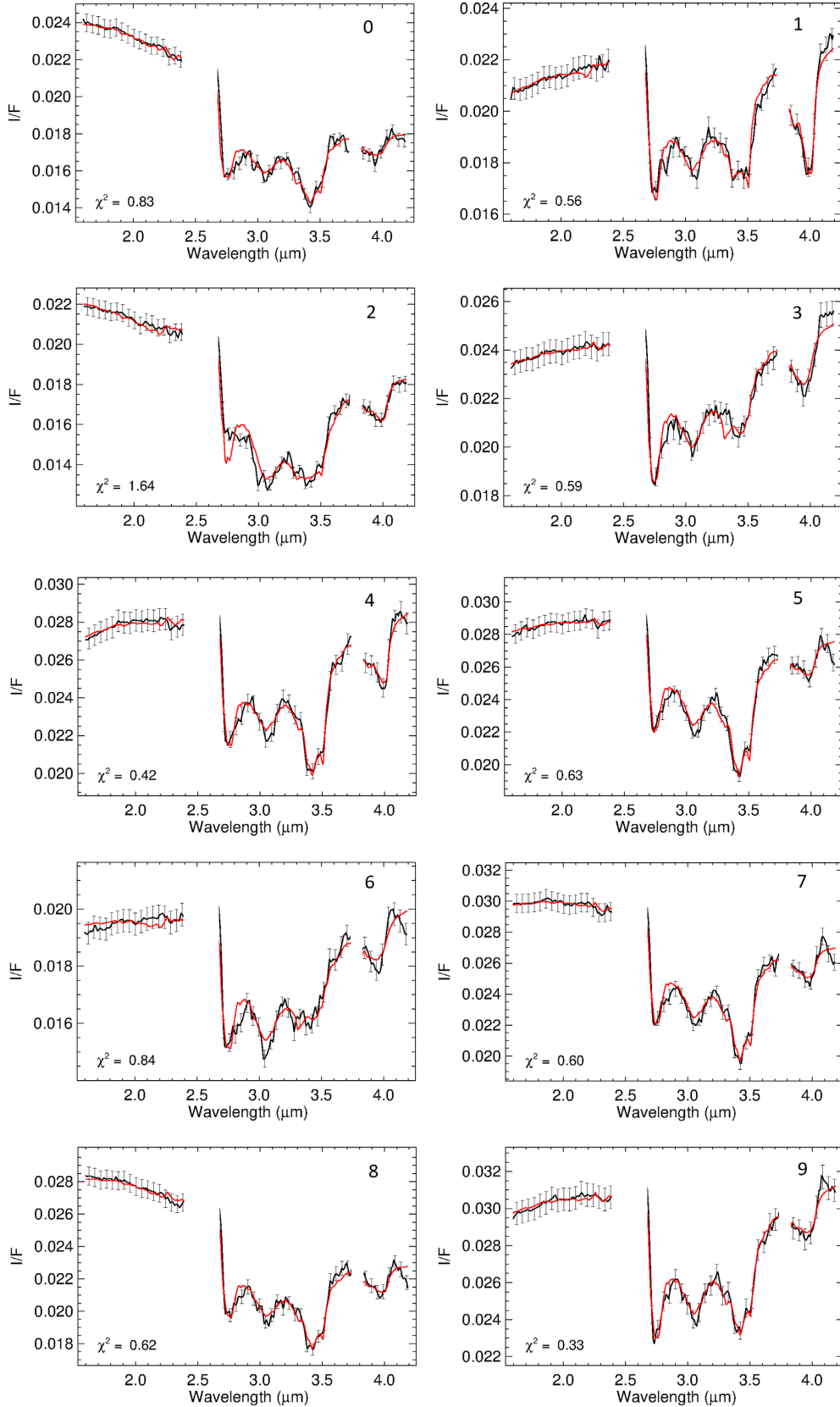
Figure 10. Spectral fits of the areas identified in Fig. 3, using the end members described in Table 1. The end member used to represent the organic component is kerite_1 (Table 1). Y-axis: radiance factor ( \pi \times reflectance) after thermal removal, hereafter called I/F . Black lines: measured spectra with error bars estimated from calibration uncertainties (Carrozzo et al. 2016). Red lines: modelled spectrum.
