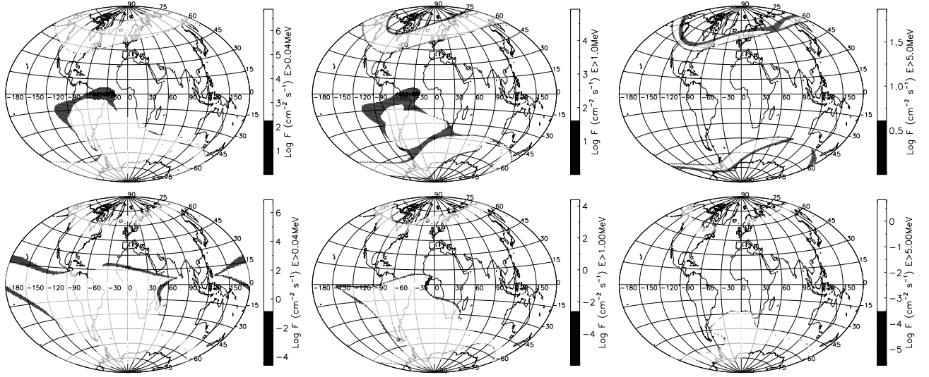
Figure 1. Integral flux maps of trapped electrons for AE8 MAX model (top panels) compared with the flux maps for AE9 50 % CL model (bottom panels) at 550 km altitude with low energy thresholds of 40 keV, 1 MeV and 5 MeV, respectively from left to right.
