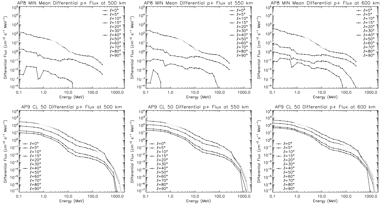
Figure 4. Orbit averaged differential fluxes of trapped protons for mean AP8 MIN (top panels) and AP9 50 % CL (bottom panels) models computed for altitudes 500, 550 and 600 km altitudes, respectively, from left to right and for different orbital inclinations I .
