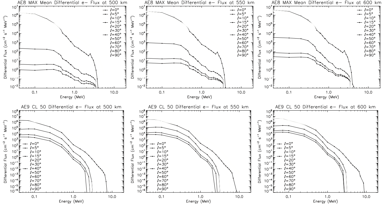
Figure 3. Orbit averaged differential fluxes of trapped electrons for mean AE8 MAX (top panels) and AE9 50 % CL (bottom panels) models computed for altitudes 500, 550 and 600 km altitudes, respectively, from left to right and for different orbital inclinations I .
