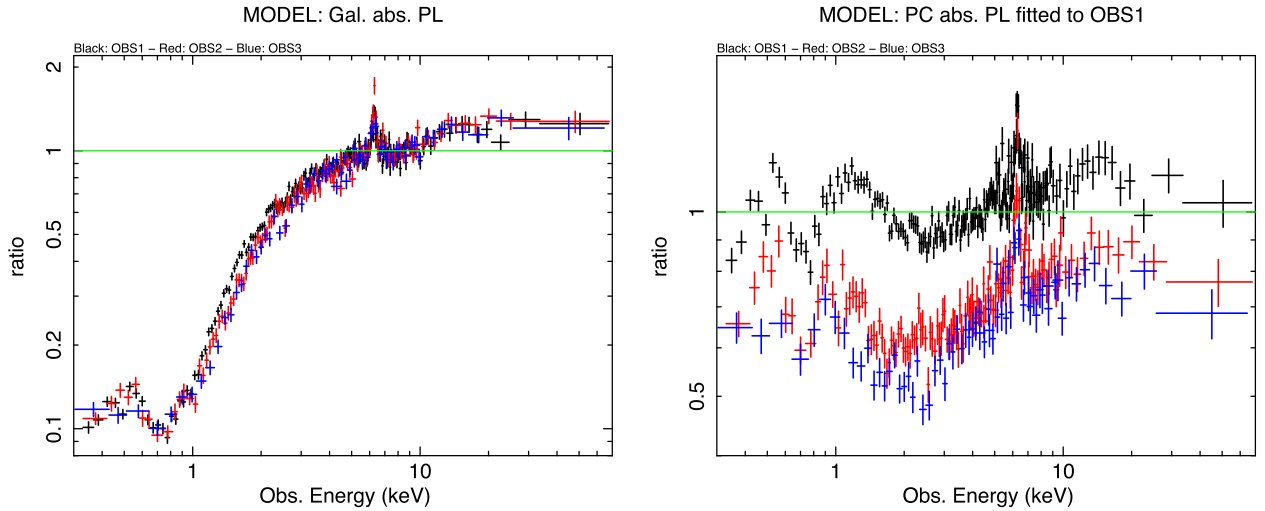
Figure 4. The data-to-model ratio for the XMM–Newton pn and NuSTAR FPMA spectra: black, OBS 1; red, OBS 2; blue, OBS 3. All data are rebinned for clarity. Left: the model is a power law, fitted to the data between 5 and 10 keV ( \Gamma \sim 1.53 ), absorbed by our Galaxy. Right: a partial covering neutral absorber is added to the model and fitted to the OBS 1 data considering the whole energy range.
