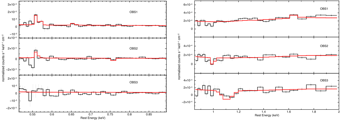
Figure 3. RGS spectra (OBS 1, top; OBS 2, middle; OBS 3, bottom) fitted with the model including an absorbed power-law continuum with the detected absorption and emission lines superimposed. The data are plotted in the source rest frame, between 0.5 and 0.9 keV (left), and between 0.85 and 2 keV (right).
