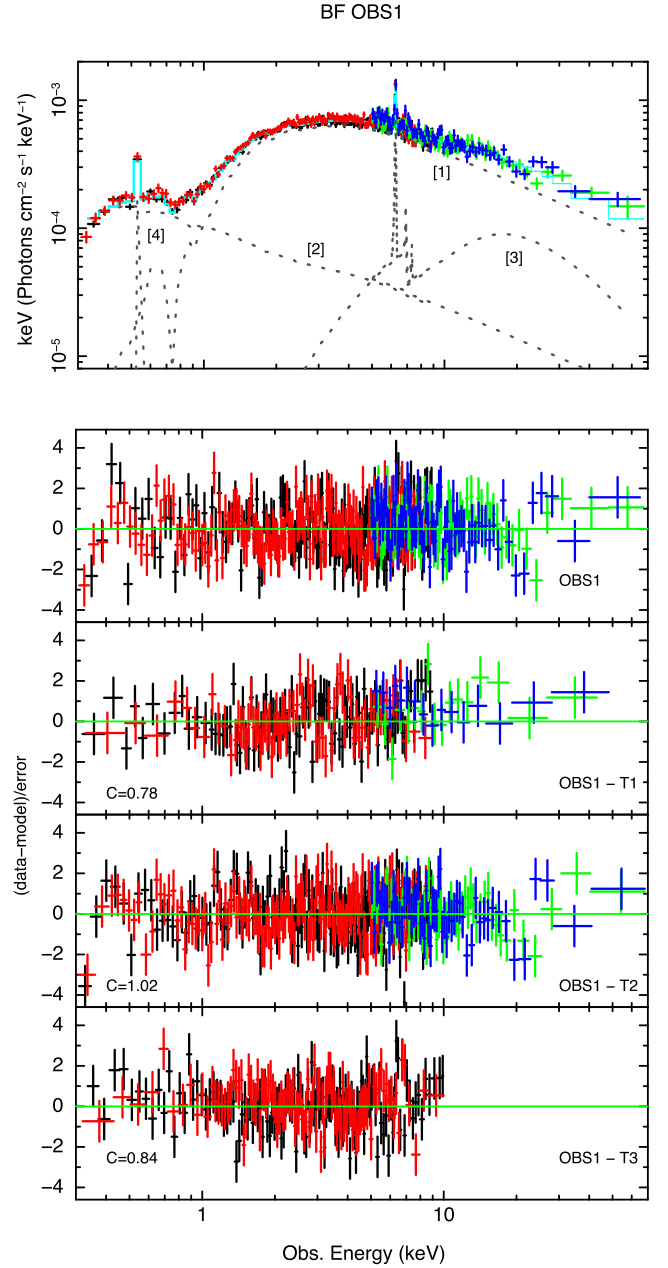
Figure 6. Upper panel: unfolded XMM–Newton (black, pn; red, MOS) and NuSTAR (green, FPMA; blue, FPMB) spectra of Mrk 915 as recorded during the whole OBS 1 period, with the best-fitting model applied (cyan continuous line): intrinsic power law partially covered by a warm absorber ([1] and [2] identify the fraction of continuum covered and uncovered, respectively) seen through a second ionized layer of material, plus reflection from distant material [3] and narrow emission line [4]; the whole emission is absorbed by neutral material partially covering the central region. Lower panels, from top to bottom: relevant residuals, plotted in terms of sigmas with error bars of size one, when the model is applied to the spectra observed during the whole OBS 1 period (same as in Fig. 5, panel d), and to the three time intervals marked in Fig. 1 (as labelled), assuming a change in the intensity of the intrinsic continuum of a factor C (with respect to the mean spectrum).
