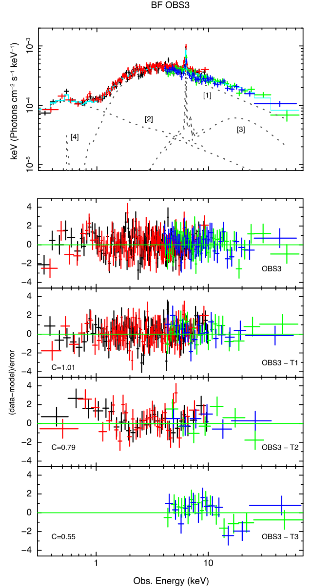
Figure 8. As in Fig. 6, but for the OBS 3 period.
