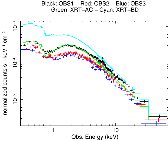
Figure 9. XMM-Newton and NuSTAR spectra (black, OBS 1; red, OBS 2; blue, OBS 3) compared with the two emission states observed during the Swift -XRT monitoring, as analysed in Severgnini et al. (2015, green, low state; cyan, high state).
