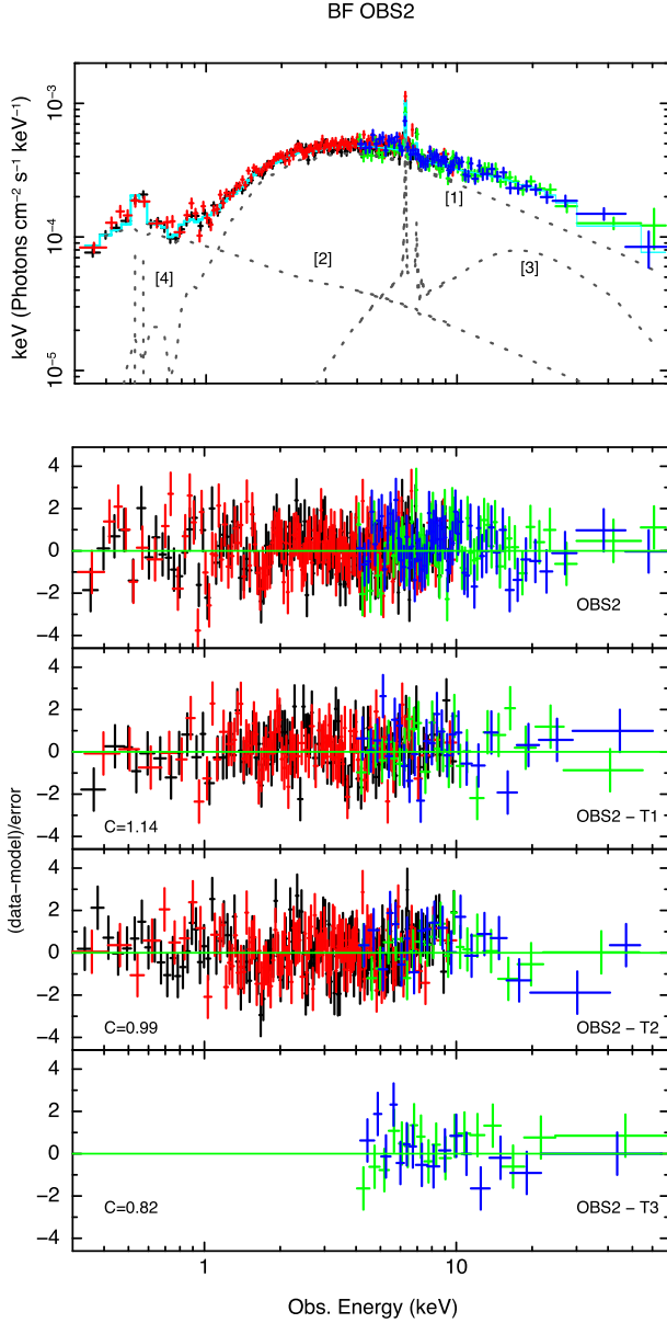
Figure 7. As in Fig. 6, but for the OBS 2 period.
