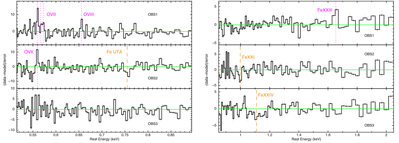
Figure 2. Residuals in the RGS OBS 1 (top), OBS 2 (middle) and OBS 3 (bottom) spectra against the continuum model (from Severgnini et al. 2015, applied to the EPIC+ NuSTAR data). The data are plotted in the source rest frame, between 0.5 and 0.9 keV (left), and between 0.85 and 2 keV (right). The vertical lines mark the positions of the emission (dotted magenta lines) and absorption (orange dashed lines) features detected during the analysis.
