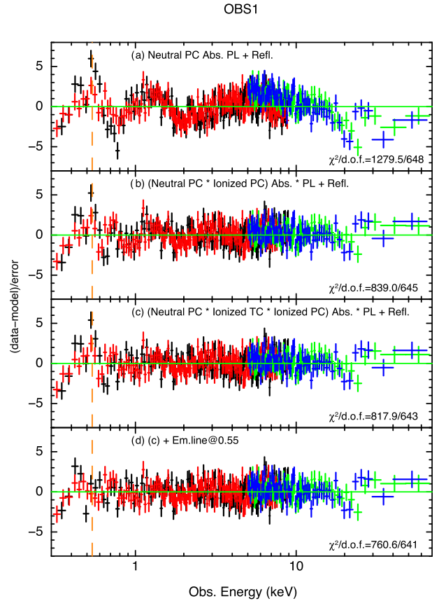
Figure 5. Relevant residuals, plotted in terms of sigmas with error bars of size one, when different models are applied to the XMM-Newton (black, pn; red, MOS) and NuSTAR (green, FPMA; blue, FPMB) spectra of Mrk 915 as recorded during the OBS 1 observation: from top to bottom, a continuum composed by the intrinsic power law and a reflection component is viewed through a partially covering neutral absorber (panel a); in panel (b) we present the residuals when a partially covering ionized absorber is included, while in panel (c) a second ionized layer has been added. Finally, panel (d) shows the residuals when the model also includes the soft X-ray emission line; its position is marked in all panels with a vertical orange dashed line. All data are rebinned for clarity.
