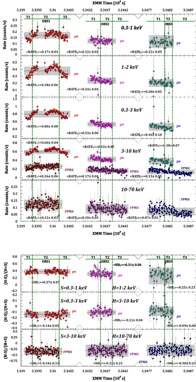
Figure 1. Background-subtracted light curves of Mrk 915 from the XMM–Newton pn and the NuSTAR FPMA observations (labeled as ‘OBS 1’, ‘OBS 2’ and ‘OBS 3’; green horizontal lines). Similar results are obtained if we consider the NuSTAR camera FPMB instead of FPMA, and/or the EPIC-MOS data instead of the EPIC-pn. For each data set, we report the mean rate (grey horizontal dashed line) and the standard deviation (shaded area) for the whole observation. The vertical green dashed lines mark the intervals (T1, T2 and T3) in which each observation has been divided (see Section 3 and Section 4). Up : count rates. From top to bottom: 0.3–1, 1–2 and 0.3–3 keV (pn only); 3–10 keV (both cameras); 10–70 keV (FPMA only). Down : hardness ratios HR = [RATE(H) - RATE(S)] / [RATE(H) + RATE(S)] . Upper panel: H = 1-2 keV and S = 0.3-1 keV (pn only); middle panel: H = 3-10 keV and S = 0.3-3 keV (pn only); lower panel: H = 10-70 keV and S = 3-10 keV (FPMA only).
