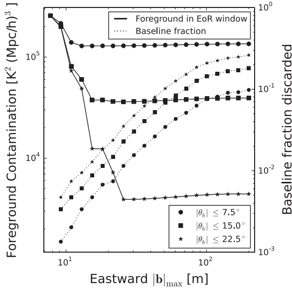
Figure 11. Drop in foreground contamination in the MWA EoR window, and loss of data for the off-zenith pointing as a function of discarded baselines. Eastward baselines with varying degrees of directedness— |\theta_b| < 7.5^\circ (solid circles), |\theta_b| < 15^\circ (solid squares), and |\theta_b| < 22.5^\circ (solid stars)—and lengths |b| \leq |b|_{\max} (x-axis) are discarded. Loss of data (dotted lines) is measured by discarded baselines as a fraction of the total number for the corresponding cases. Foreground contamination in the EoR window (solid lines) drops by a factor of \sim 2 ( |\theta_b| \leq 7.5^\circ ) to \sim 100 ( |\theta_b| \leq 22.5^\circ ). The latter limit can be achieved with a mere 5% loss of data at |b|_{\max} \simeq 30 m, and discarding longer baselines ( |b| \gtrsim 30 m) has no effect in further reducing foreground contamination.
