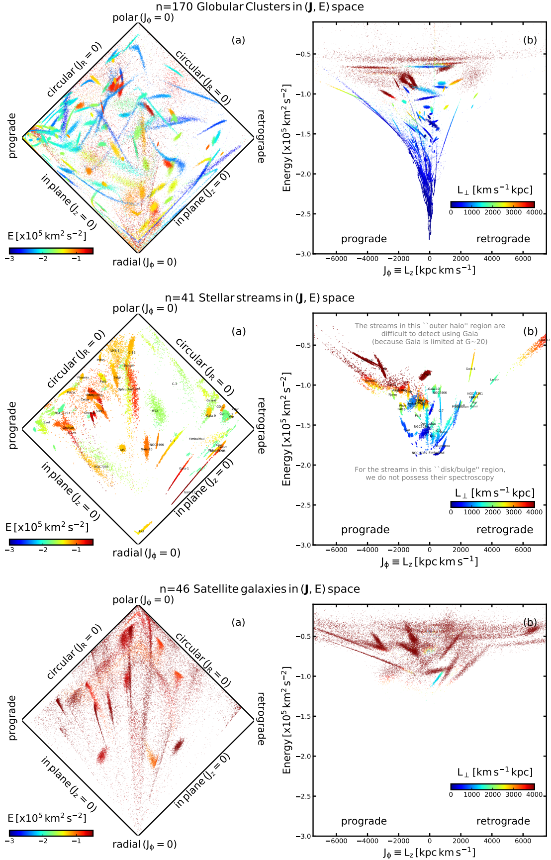
Figure 2. Action-Energy (J, E) space of the Milky Way showing globular clusters (top panels), stellar streams (middle panels) and satellite galaxies (bottom panels). Each object can be seen as a ‘cloud’ of 1000 Monte Carlo representations of its orbit (see Section 2.2). In each row, the left panel corresponds to the projected action-space map, where the horizontal axis is J_\phi/J_{\text{tot}} and the vertical axis is (J_z - J_R)/J_{\text{tot}} with J_{\text{tot}} = J_R + J_z + |J_\phi| . In these panels, the points are colored by the total energy of their orbits ( E ). The right panels show the z -component of the angular momentum ( J_\phi \equiv L_z ) vs E , and the points are colored by their orthogonal component of the angular momenta ( L_\perp = \sqrt{L_x^2 + L_y^2} ).
