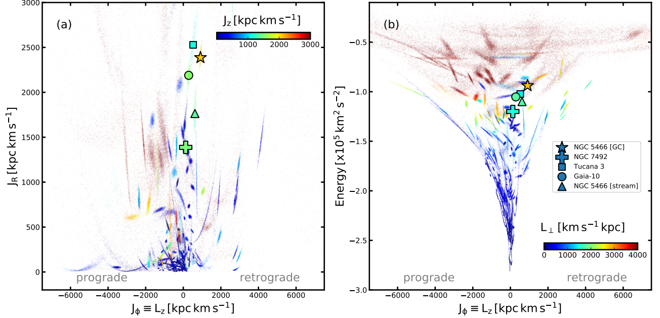
Figure 10. (J, E) distribution of the objects belonging to the candidate merger (see Section 5). These objects are shown along with all the other objects in our sample. Similar to Figure 2, each object is shown as a ‘cloud’ of 1000 Monte Carlo representations of its orbit.
