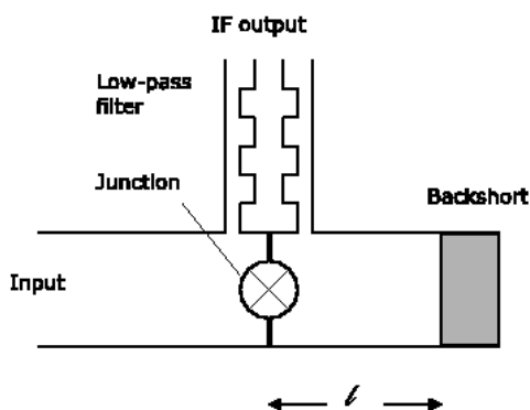
Fig. 2.3.1. A sketch of a SIS mixer.
