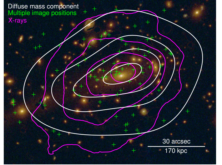
Fig. 4: Cluster members of MACS 1206 used in the strong lensing models. Galaxies that do not satisfy the selection criteria described in Sec. 3.2.1 have been masked out of the original HST image using the SExtractor segmentation map. The white lines show the contour levels of the reconstructed surface mass density of the diffuse mass components only (obtained by removing the surface mass density of the cluster member halos from that of the total), corresponding to the values of [1.0, 1.5, 2.0, 3.0] \times 10^{15} \text{ M}_\odot \text{ Mpc}^{-2} . The magenta lines show the isocontours of the 0.5 – 7 keV Chandra X-ray detection. The green crosses indicate the positions of the multiple images shown with white and green circles in Figure 1.
