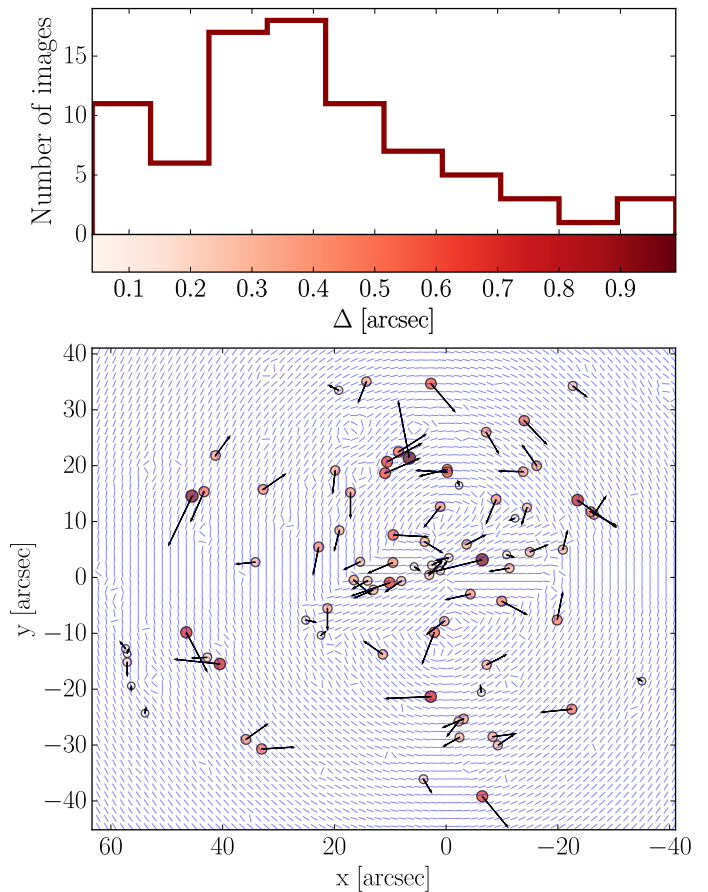
Fig. 5: Offset between the observed and model-predicted (model ID P3ε in Table 1) positions of the multiple images in MACS 1206. Darker hues of red correspond to larger offsets. In the top panel, the histogram shows the distribution of the absolute values of the differences ( \Delta ). In the bottom panel, the circles indicate the observed positions of the multiple images, and the arrows point towards the model-predicted positions. For the sake of clarity, the arrow lengths are ten times larger than the values of the corresponding offsets. The blue sticks represent the shear orientation on a regular grid (see Sect. 3.1) for a source at z_{src} = 1.4 .
