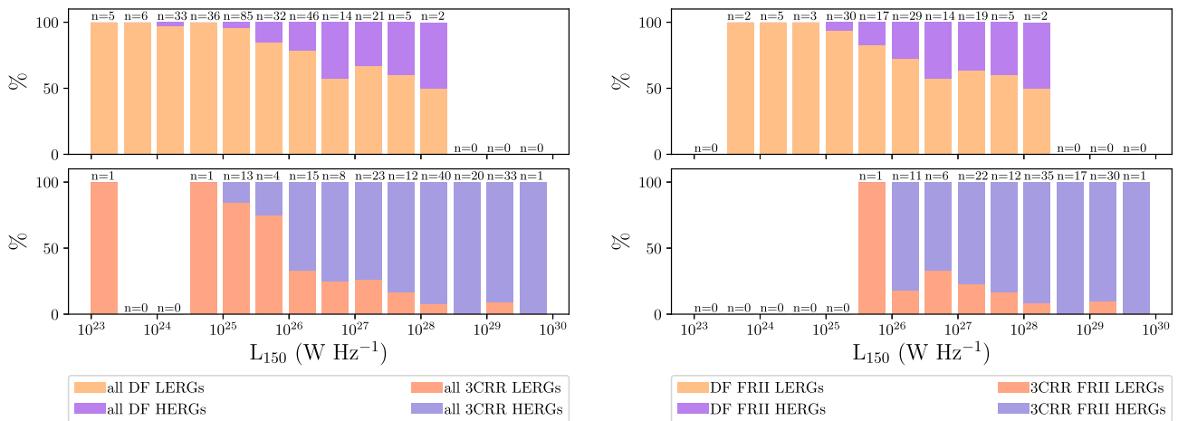
Figure 7. Left: Stacked histograms showing the percentile fraction of LERGs and HERGs in our LoTSS-Deep data set (top) and the 3CRR sample (bottom) as a function of luminosity, regardless of their FR classification. Right: Same plot, restricted to FRII sources in both samples. In all panels LERGs are shown in shades of orange and HERGs in shades of purple. 3CRR Data obtained from M. Hardcastle’s updated version of the Laing et al. (1983) 3CRR catalogue (available at https://3crr.extragalactic.info/ ). 3C 343.1 was excluded from the sample (Arp, Burbidge & Burbidge 2004).
