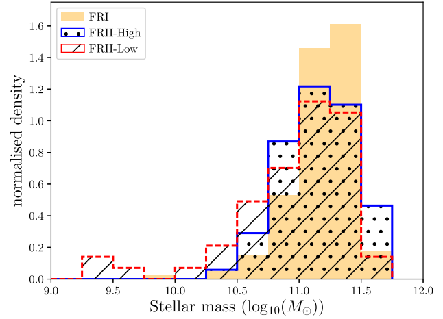
Figure 14. Normalized histogram distribution of stellar masses for the LoTSS-Deep FRI (yellow, solid), FRII-High (blue solid outline, dotted), and FRII-Low (red dashed outline, hashed).
