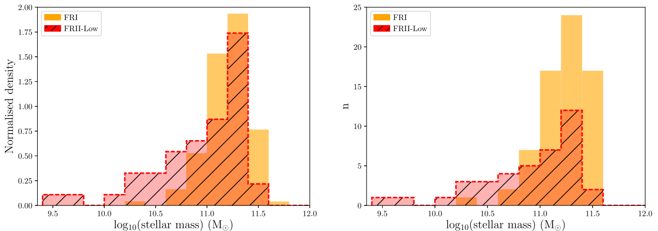
Figure 15. Stellar mass distributions for a subset of matched FRI (yellow solid bars) and FR II-Low (red hatched bars, dashed outline). Left (normalized): Samples matched in size and luminosity ( 200\text{--}1000 kpc, 24.3 < \log_{10}(L_{150}) < 26 W Hz ^{-1} ). Right: Narrower luminosity range, focusing on the sources just below the traditional FRI/II boundary ( 25 < \log_{10}(L_{150}) < 26 W Hz ^{-1} ).
