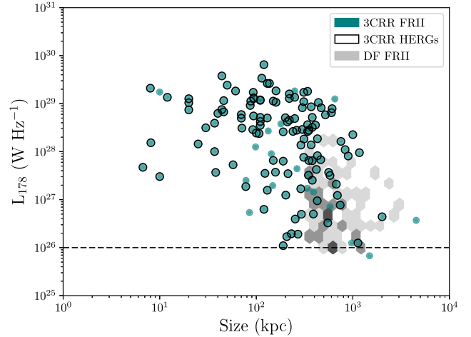
Figure 12. Luminosity versus size distribution for all the FR II sources in the 3CRR survey. Empty black circles surround the HERGs. The plot also shows a density map of the DF FR IIs (regardless of accretion mode), with darker shades of grey denoting larger numbers of sources in a given hexagonal bin.
