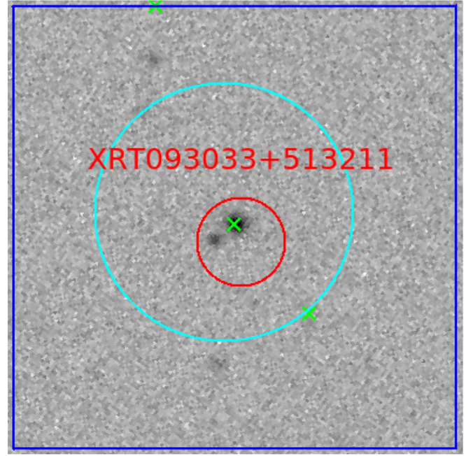
Figure 1. Optical images of the proposed counterparts of the \gamma -ray sources. The images are taken from the SDSS ( g filter) or DSS survey ( B filter), field = 60 arcsec \times 60 arcsec, north up, east left. Details of the optical counterparts are reported in Table 1. The red circles represent the error box of the proposed X-ray counterparts of the \gamma -ray sources found with Swift /XRT data (magenta circles indicate an X-ray source of the ROSAT catalog), the cyan circles the radio counterparts (see the details in Section 1), and the green crosses the WISE IR counterparts. The optical image of 3FGLJ2246.2+1547 is displayed in Paper I. (The complete figure set (27 images) is available.)
