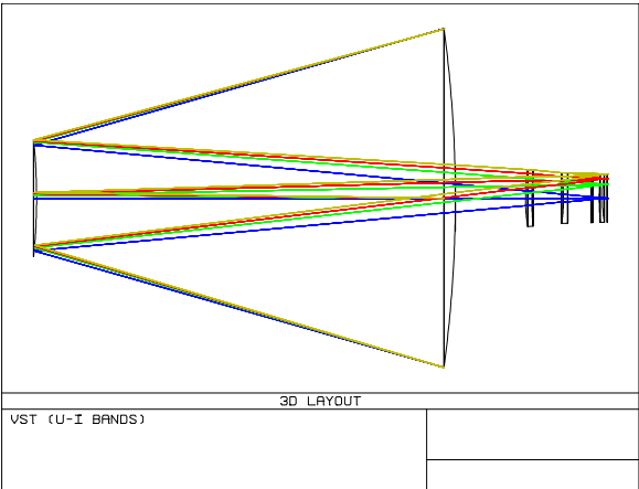
Fig. 3 - Optical layout of telescope with two - lens corrector (U + I bands) with a curve dewar window
