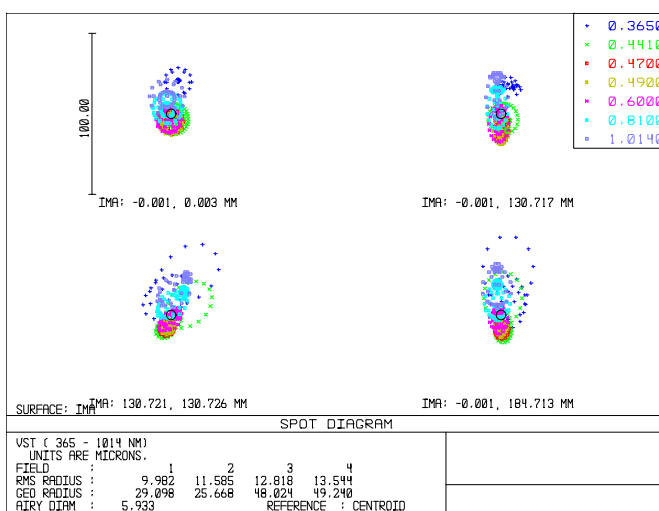
Fig.10 – Spot with ADC correction at 60° z angle
