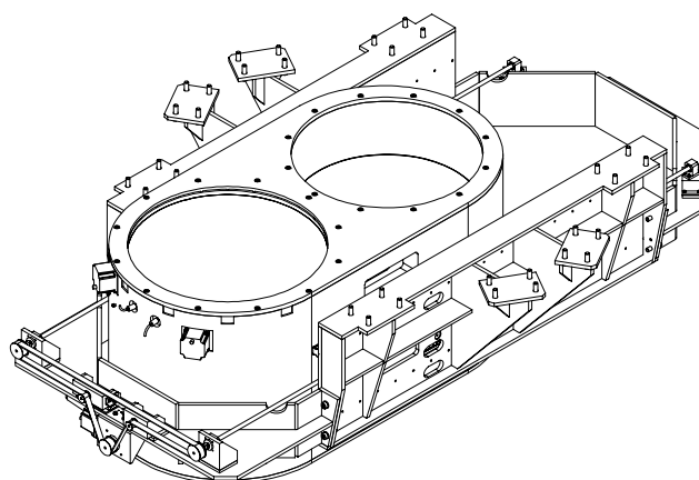
Fig. 7 – Corrector Support 3D view side
