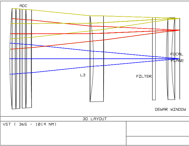
Fig. 5 - ADC and one-lens corrector optical layout
