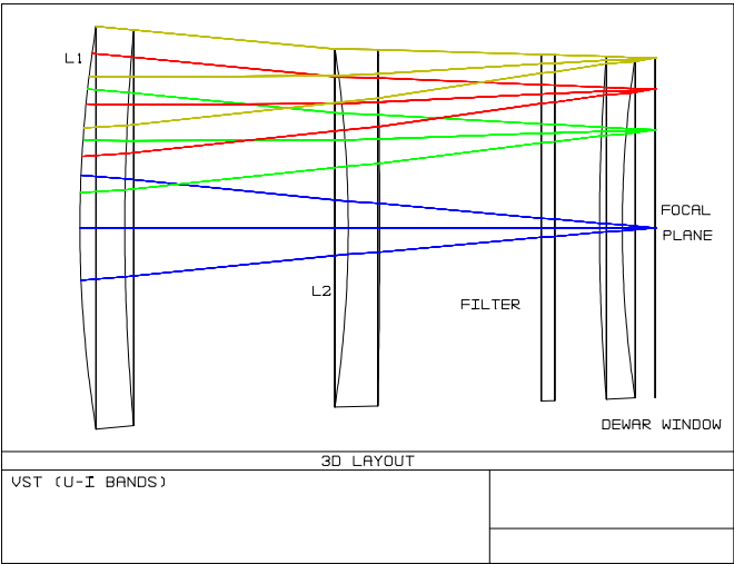
Fig. 4 – Two-lens corrector optical layout
