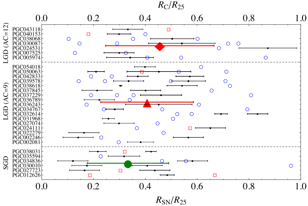
Figure 4. Galactocentric positions of normalized corotation radii (black points) and their errors for 30 host galaxies of Table 4. SGD (AC = 5 and 6), LGD (AC = 9), and LGD (AC = 12) galaxies are separated by horizontal dashed lines. The filled diamond, triangle, and circle are the corresponding mean values of the corotation radii (with their standard deviations). For each host galaxy, galactocentric positions of Type Ia (red empty squares) and CC (blue empty circles) SNe are also presented. In PGC 050063, one of the CC SNe is located at R_{SN}/R_{25} = 1.59 and not shown in the plot.
