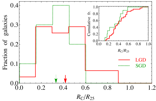
Figure 5. Histograms and cumulative distributions (inset) of R_C/R_{25} values of LGD (red solid) and SGD (green dotted) galaxies. The mean values are shown by arrows.
