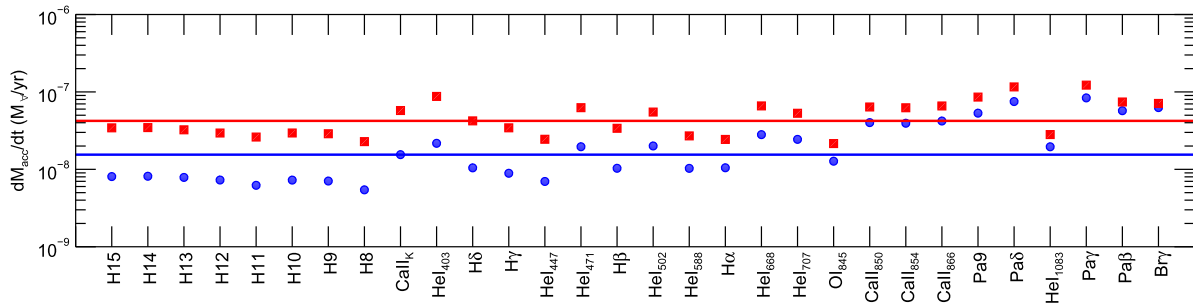
Figure 3. Mass accretion rate determination computed from the flux of the labeled tracers using Alcalá et al. (2014) relationships. The assumed visual extinction is A_V = 1 mag (blue circles) and A_V = 2 mag (red squares). The median \dot{M}_{\text{acc}} values are marked for both cases with a solid line.
