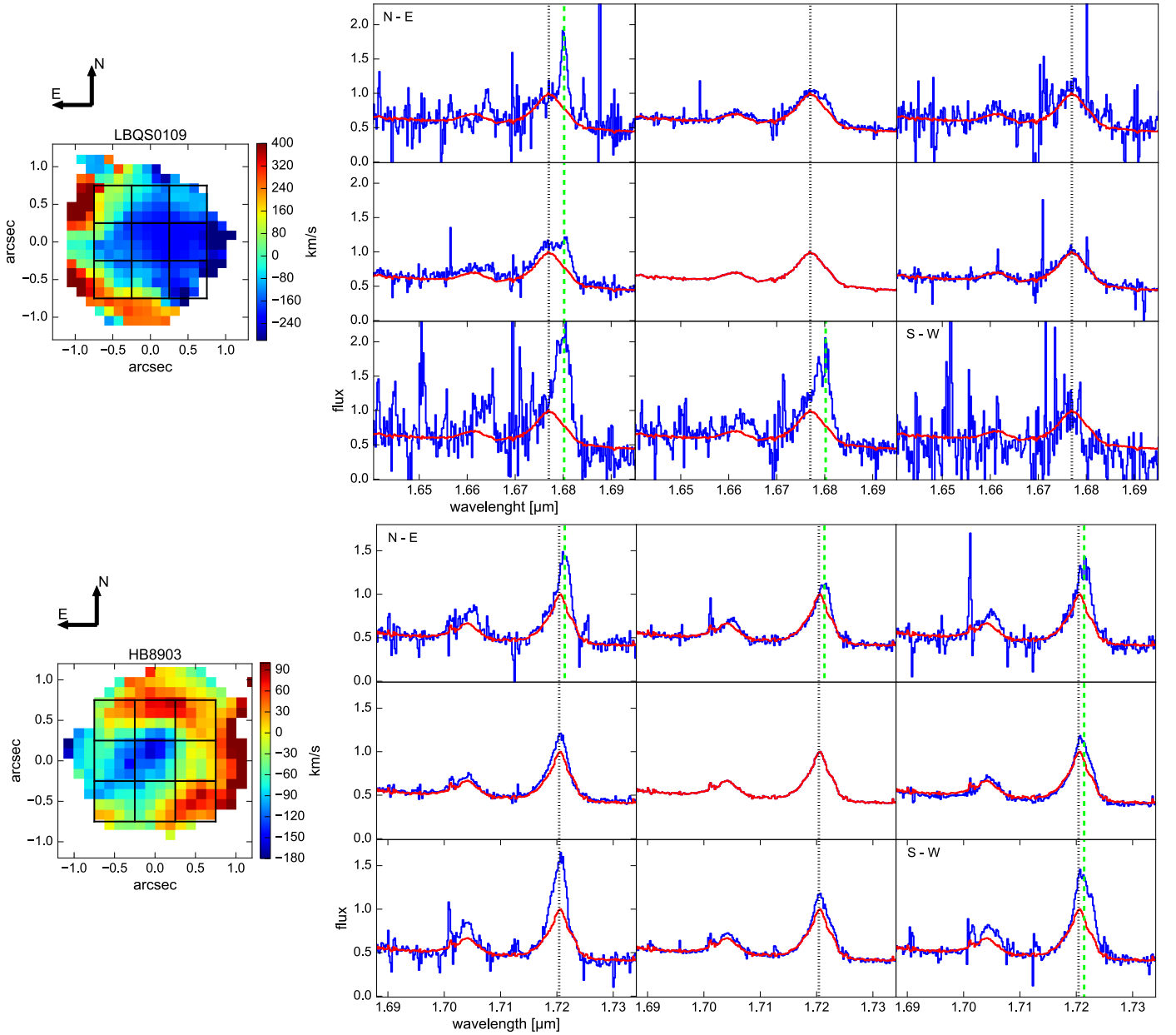
Fig. 1. Left panels: [\text{OIII}]\lambda 5007 velocity maps of LBQS0109 (top) and HB8903 (bottom) presented in Paper I. Black squares indicate the nine regions where we extracted the corresponding spectra shown in the right panels. Right panels: comparison between the nuclear [\text{OIII}]\lambda 5007 profiles (red) and those from the external regions (blue) of LBQS0109 (top) and HB8903 (bottom). The black dotted line corresponds to the [\text{OIII}]\lambda 5007 central wavelength. Narrow ( FWHM \sim 490 \text{ km s}^{-1} for LBQS0109 and FWHM \sim 480 \text{ km s}^{-1} for HB8903) components of the [\text{OIII}]\lambda 5007 emission, identified by the green dashed line, are clearly detected.
