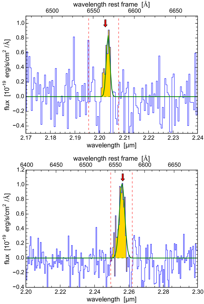
Fig. 6. Narrow H\alpha emission from the residual K -band fitting, extracted from a ring-shaped region ( 0.5'' < r < 0.8'' ) of LBQS0109 (top) and HB8903 (bottom). The red arrows indicate the expected position at the redshift of the [OIII]_{\text{nar}} component. The dashed red line indicates the expected positions for doublet [NII] ; the lines are not detected, confirming that star formation is the excitation mechanism for the narrow H\alpha line (see text).
