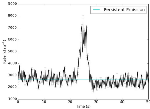
Figure 12. A representative RXTE light curve of a Miniburst from OBSID 20077-01-03-00 in Outburst 2.
