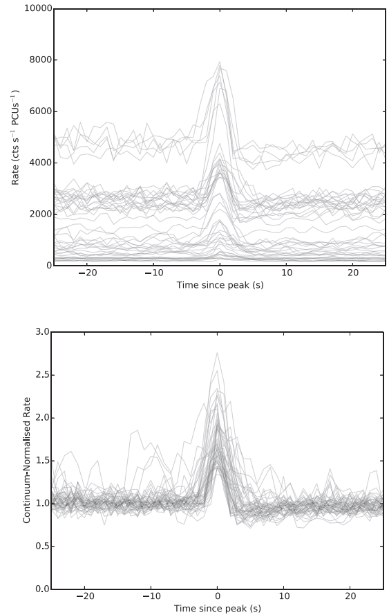
Figure 13. Top: a plot of every Miniburst, centred by the time of its peak, overlaid on top of each other. Bottom: a plot of every Miniburst in which count rates have been normalized by the persistent emission count rate during the observation from which each burst was observed.
