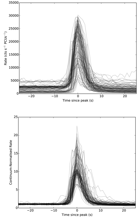
Figure 7. Top: a plot of every Normal Burst, centred by the time of its peak, overlaid on top of each other to show the existence of a common pulse profile. Bottom: a plot of every Normal Burst in which count rates have been normalized by the persistent emission count rate during the observation from which each burst was observed. As the bursts are on average closer to the average pulse profile in this metric, this suggests that the intensity of a burst is roughly dependent on the persistent emission rate. Some persistent emission-normalized count rates may be artificially low due to dead-time effects.
