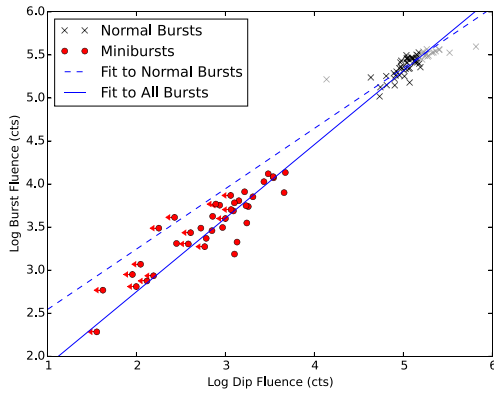
Figure 22. A scatter plot showing the relationship between burst fluence and ‘missing’ dip fluence for Normal Bursts (black) and Minibursts (Red), with the best-fitting power law plotted in solid blue. A power-law fit to just the Normal Bursts (blue dashed line) also approaches the Minibursts. Note that the Normal Bursts plotted in grey were not used to calculate this latter fit, as the effects of instrumental dead time cause high burst fluences to be underreported. Upper limits on Miniburst dip fluences are shown with arrows.
