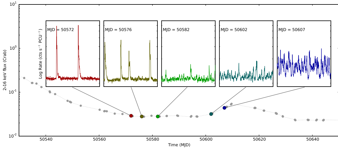
Figure 20. A series of light curves from RXTE /PCA observations of Outburst 2, showing a gradual evolution from Mesobursts to Structured Bursting over a period of \sim 30 d. Each inset light curve is plotted with the same y-scaling, and each corresponds to 2 ks of data.
