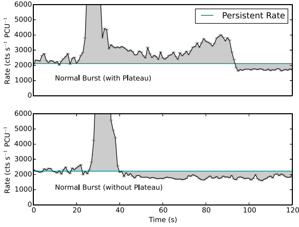
Figure 8. RXTE light curves of Normal Bursts with (top) and without (bottom) ‘plateau’ features, showing the burst structure in each case. The median count rate, which we use as a proxy for the persistent emission, is plotted in cyan to highlight the presence of the count rate ‘dip’ after each burst.
