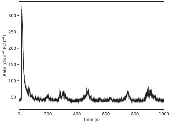
Figure 17. A light curve from RXTE /PCA observation 10401-01-57-03, showing a Mesoburst occurring during a period of Structured Bursting.
