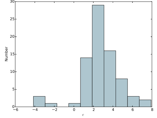
Figure B4. A histogram showing the distribution of burst skewness c amongst our sample of Normal Bursts.
