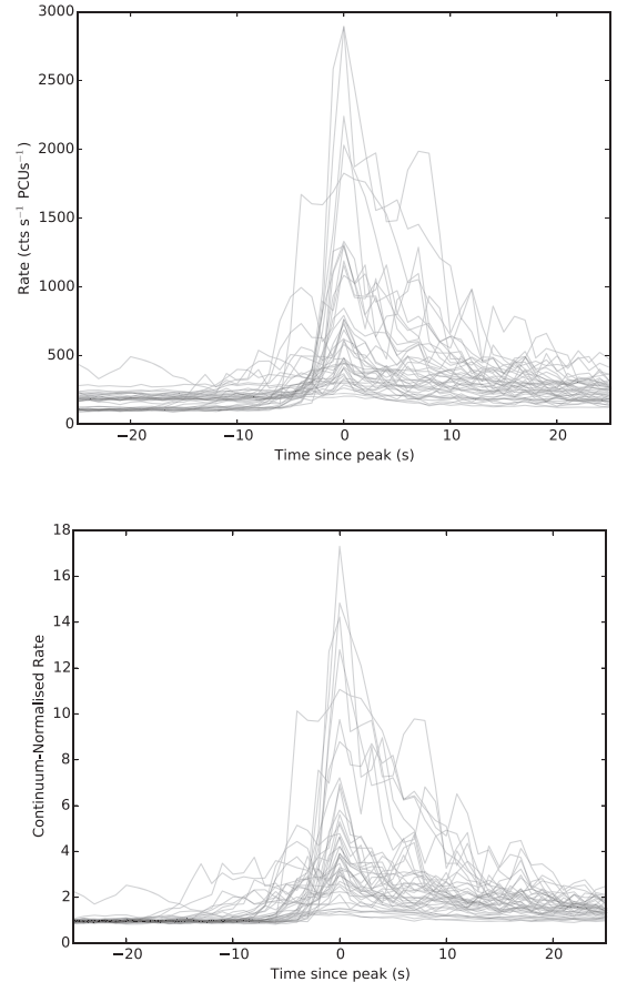
Figure 16. Top: a plot of every Mesoburst, centred by the time of its peak, overlaid on top of each other. Bottom: a plot of every Mesoburst in which count rates have been normalized by the persistent emission count rate during the observation from which each burst was observed.
