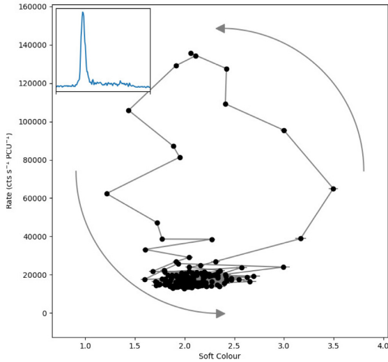
Figure 11. A 1 s-binned hardness-intensity diagram of a Normal Burst from RXTE /PCA observation 10401-01-08-00, with an inset 2–60 keV light curve. Significant colour evolution can be seen during the burst, taking the form of a loop.
