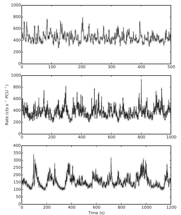
Figure 19. A selection of RXTE light curves from Structured Bursting observations of the Bursting Pulsar. Top: a light curve from Outburst 1 showing flaring on time-scales of \sim 10 s. Middle: a light curve from Outburst 1 showing the same flaring behaviour with an additional slower modulation over \sim 50 s. Bottom: a light curve from Outburst 2 showing a regular sequence of flat-bottomed dips and multi-peaked flaring. These show the wide variety of variability patterns that we classify as ‘Structured Bursting’.
