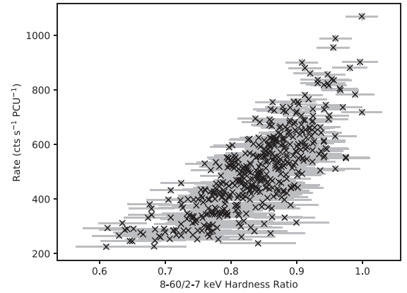
Figure 18. A 1 s-binned hardness-intensity diagram from RXTE observation 20078-01-23-00, showing that hardness tends to correlate with intensity during Structured Bursting. Data are binned to 8 s, and background has been estimated by subtracting mean count rates in the relevant energy bands from RXTE OBSID 30075-01-26-00.
