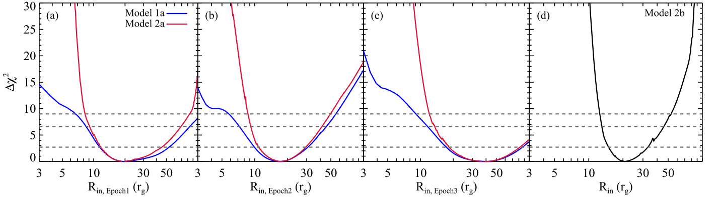
Figure 5. \Delta\chi^2 contours of the inner disk radius R_{\text{in}} obtained from Models 1a, 2a, and 2b. The dashed lines indicate the 90%, 99%, and 3\sigma confidence levels for one parameter of interest.
