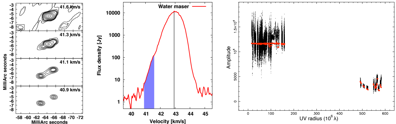
Figure 4. (Center) A logarithmic scale spectrum highlighting the bursting maser feature, in which the peak channel is indicated with a grey line and the blue wing is coloured. (Left) Channel maps of the blue wing convey the structure of the emission with contours at 1, 2, 3, 4, 5, 10, 20, 40, 80, 160 multiples of 0.5 Jy which is a typical 3\sigma noise value in the off-peak channels. Coordinates are relative to the reference maser spot. (Right) A plot of amplitude as a function of projected baseline length for the peak maser channel (black) and a linear model with a Gaussian flux density profile (red) indicating structure at sub-/milliarcsecond scale.
