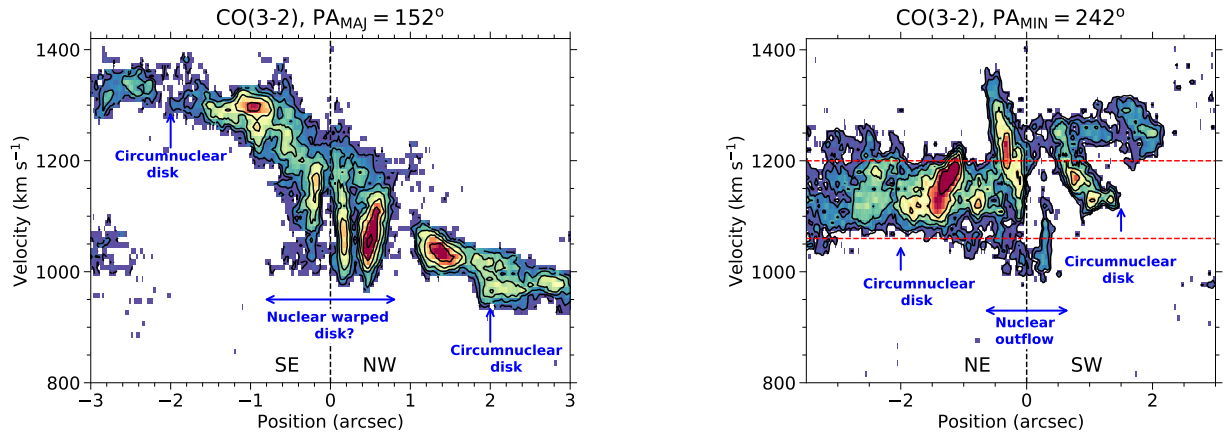
Fig. 9. Observed CO(3-2) p-v diagrams along the kinematic major axis ( left ) and minor axis ( right ) of the host galaxy disk. We only show fluxes above 3\sigma . The black contours are fluxes in a linear scale. The black dotted vertical line marks the AGN position, whereas the horizontal red lines mark the approximate velocity virial range of the simple rotating disk model (see top panel of Fig. 8).
