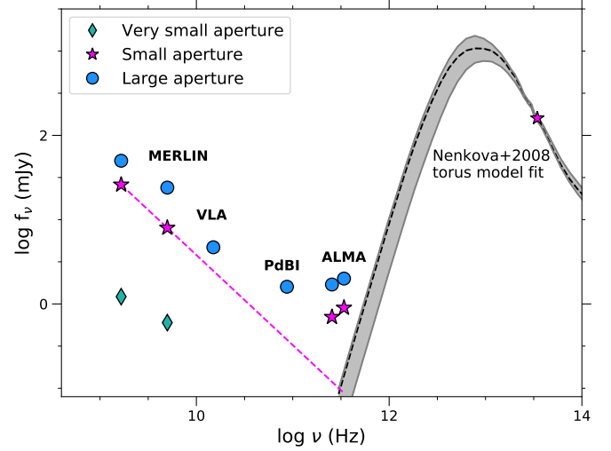
Fig. 4. Nuclear continuum SED from centimeter wavelengths to the infrared of NGC 3227. The small-aperture ( \sim 0.1 – 0.2'' ) MERLIN data points are for the southern source of Mundell et al. (1995b). The large-aperture ( >0.2'' to \leq 1'' ) VLA and PdBI data points are from Nagar et al. (2005) and Sani et al. (2012), respectively. All the ALMA continuum data points are from this work. The very small aperture (a few milli-arcseconds) points are the EVN radio fluxes from Bontempi et al. (2012). The fit (black dashed line, with the \pm 1\sigma uncertainty plotted with the shaded gray region) is made to the near- and mid-infrared emission using the Nenkova et al. (2008a,b) clumpy torus models (see García-Bernete et al. 2019, for more details). We also plot the observed mid-infrared data point for reference although the fitted data also included near-infrared photometry and mid-infrared spectroscopy. The magenta dashed line is the fit to the MERLIN radio points extrapolated to the ALMA wavelengths.
