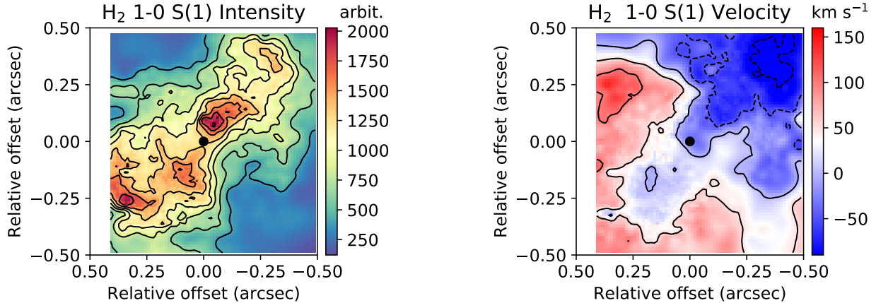
Fig. 6. VLT/SINFONI H 2 1–0 S(1) intensity (left) and velocity (right) maps from Davies et al. (2006) showing a FoV similar to that of Fig. 5. The maps were derived by fitting a Gaussian to the emission line. The black dot marks the approximate location of the peak of the near-infrared continuum. The velocities are relative to this peak. To facilitate the comparison with the CO(2–1) and CO(3–2) emission, we show the same velocity range as in the right panels of Fig. 5.
