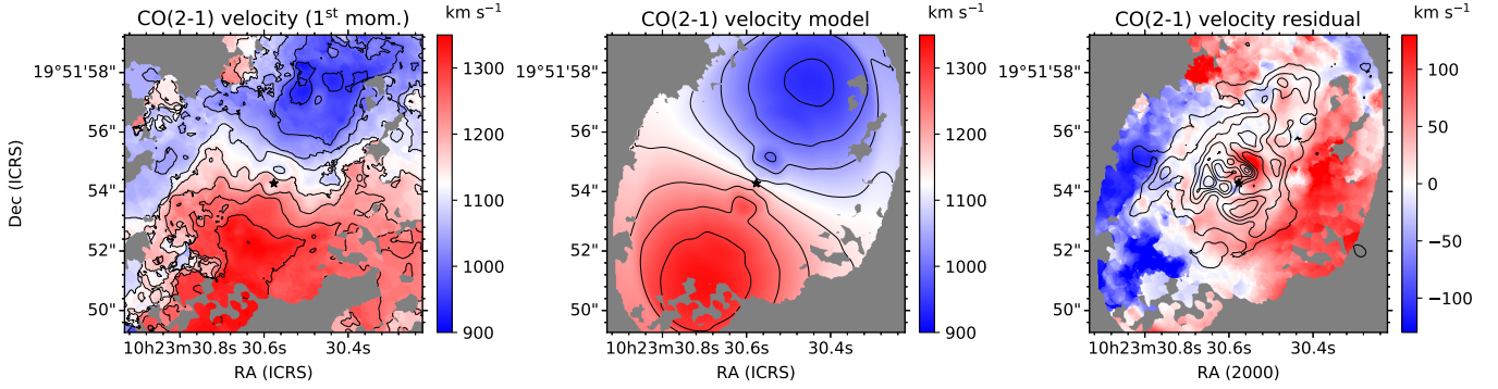
Fig. 7. ^3\text{D} BAROLO maps of the observed CO(2–1) mean velocity field (first-order moment, left panel ), the fitted model of a rotating disk with fixed PA, inclination (see Table 4 and text), systemic velocity, and kinematic center ( middle panel ), and the residual mean-velocity field ( right panel ). The FoV is 10'' \times 10'' , as in Fig. 1. The color bars indicate line-of-sight velocities in units of \text{km s}^{-1} . The contours for the velocities in the left and middle panels are in steps of 50 \text{ km s}^{-1} . Right panel : the contours are the CO(2–1) intensity (zeroth-order moment map) on a linear scale.
