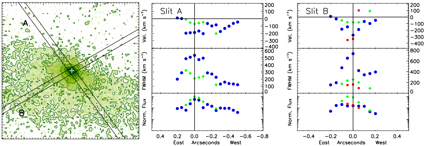
Figure 12. HST imaging observations of the nucleus of Mrk 1040. The left-hand plot shows the WPC2 image of Mrk 1040 at [O III] \lambda 5007 showing the central 2''.5 \times 2''.5 region of the galaxy centered on the AGN (white cross). North is up, east is to the left. At the distance of Mrk 1040, the scale is 330 \text{ pc arcsec}^{-1} . The position of the two slits used for the HST STIS observations (with the G430M grating) are marked A and B, respectively. Slit A is positioned along the major axis of the galaxy. The middle and right panels show the results of the kinematics obtained from the [O III] line fitting for the two slit positions vs. the position (in arcseconds) from the AGN center. The top panels show the velocity shift of the [O III] emission vs. position, where negative values denote blueshift. Thus a small component of outflow of \sim -200 \text{ km s}^{-1} is found within \pm 0''.2 of the nucleus in both of the slit A and B spectra, while a small blueshifted component is seen up to 0''.5 SW of the nucleus for slit A only—this latter component may be due to rotation. The middle panels show the FWHM of the [O III] line components we fit, while the lower panel shows the relative [O III] flux vs. position. The different colored points illustrate the kinematics of different components of [O III] selected on FWHM. Thus blue, green, and red points signify the widest, second widest, and third widest components, respectively, as can be seen from their FWHM values in the middle panels.
