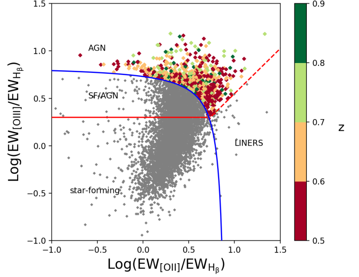
Fig. 1: Blue diagram (Lamareille 2010) for the VIMOS sample. Diamonds represent Type II AGN color-coded according to their redshift. VIMOS galaxies with reliable emission line measurements are marked with grey dots. The blue curve shows the separations between star-forming galaxies and AGN (Eq. 1), the red dashed line between AGN and LINERS (Eq. 2), the red solid line between star-forming galaxies and SF/AGN (Eq. 3).
