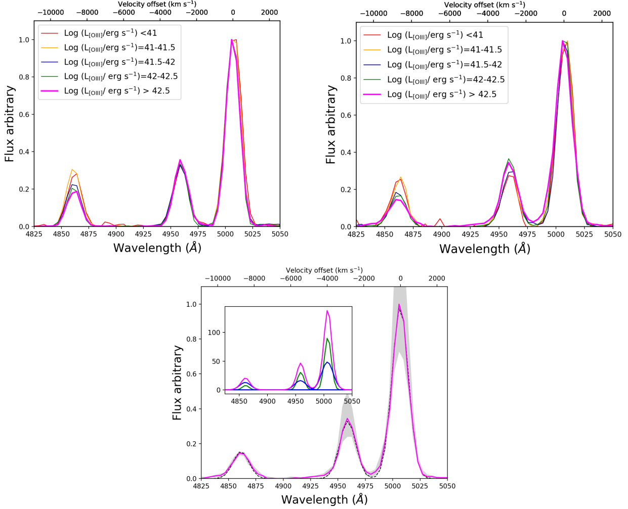
Fig. 7: Comparison of the stacked spectra, in the H\beta -[OIII] doublet lines wavelength range, in bins of [OIII] \lambda 5007 luminosity above (left) and below (right) the line threshold as defined in Sec. 4.2. (lower panel) Stacked spectrum in the [OIII] luminosity bin \text{Log}(L_{[\text{OIII}]}/\text{erg s}^{-1}) > 42.5 of the low-SF Type II AGN with superimposed the 1\sigma uncertainties estimated through a bootstrap resampling technique and the best fitting one-component Gaussian curve (black dashed line). The inset plot shows the best-fit double Gaussian model (magenta curve) and its line decomposition (green and blue Gaussian profiles refer to the narrow and broad best-fit components).
