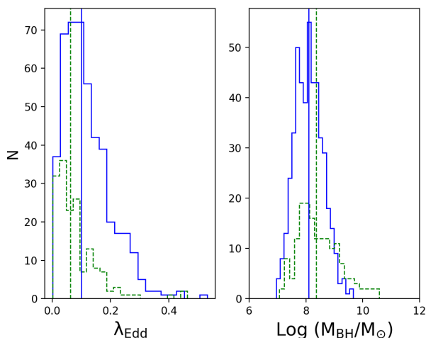
Fig. 8: Eddington ratio (left) and black hole mass (right) distributions of Type II AGN divided into two subsamples, according to the classification of their host galaxies as high-SF (blue) and low-SF (green). Solid and dashed lines represent the median value of the parameters.
