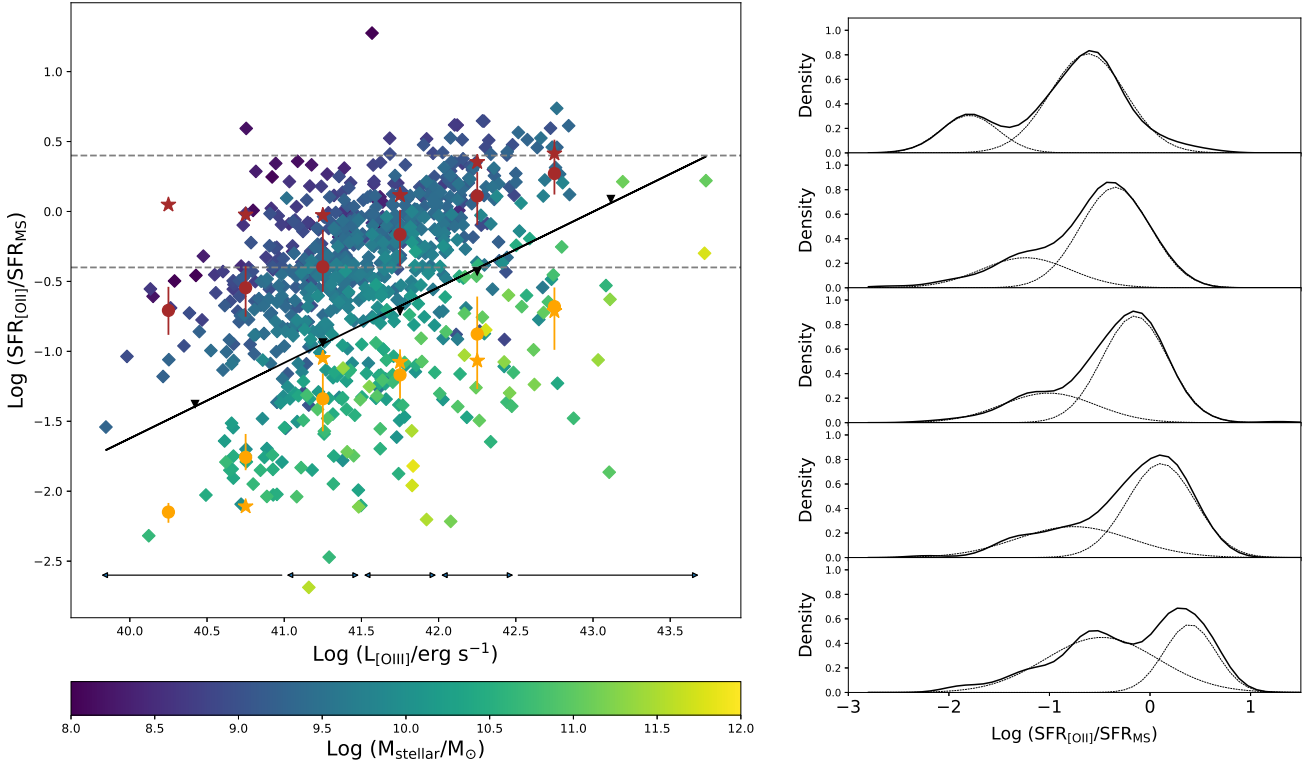
Fig. 6: (left panel) Distance from the MS (parameterised as \text{SFR}_{\text{OIII}}/\text{SFR}_{\text{MS}} ) as a function of [OIII] luminosity (proxy of AGN power) for the VIMOS sample (diamonds) color-coded according to the stellar mass. Median values of [OII]-based and SED-based SFR offset in bins of [OIII] luminosities are represented as brown and orange circles and stars, below and above the line threshold, respectively (see the main text for details). The dashed lines delimit the locus of the MS ( \pm 0.4 dex). (right panel) Probability density function of the SFR offset in each luminosity bin (black solid lines), with superimposed the best-fit Gaussian components (black dashed lines) which reproduce the observed bimodality (see Sec. 4.2).
