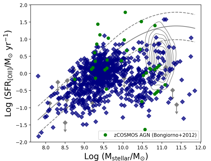
Fig. 5: Star formation rate (SFR) as a function of stellar mass ( M_{\text{stellar}} ) for the VIMOS sample (blue diamonds). The solid line represents the star-forming main sequence as found by Schreiber et al. (2015) and dashed lines mark the scatter of 0.4 dex. Upper limits are shown as grey diamonds. Optically selected Type II AGN from zCOSMOS survey as found by Bongiorno et al. (2012) and from BOSS DR12 are shown as green circles and grey contours, respectively.
