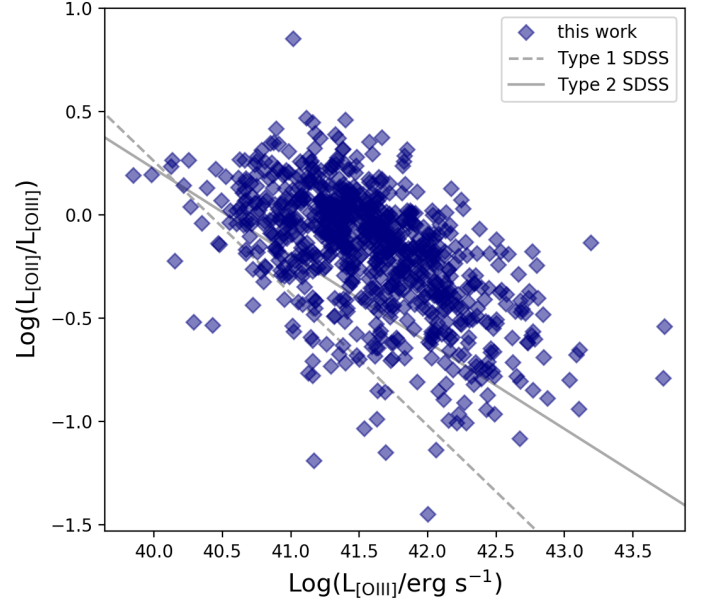
Fig. 4: [OII]/[OIII] luminosity ratio as a function of [OIII] luminosity for the VIMOS Type II AGN. Dashed and solid lines represent the best-fit relation for SDSS Type I and Type II AGN at z < 0.3 , respectively.
