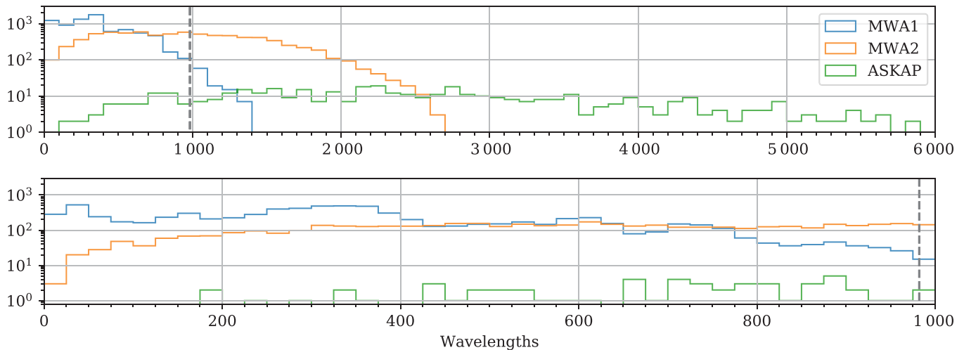
Figure 1. A comparison of baseline lengths for each of MWA Phase I (MWA1), MWA Phase 2 extended configuration (MWA2) and ASKAP. The lengths are measured in wavelengths (i.e. |b|/\lambda , with \lambda \approx 1.94 m for the MWA and \lambda \approx 0.34 m for ASKAP), which allows us to compare the baseline coverage despite the different observing frequencies. All plots exclude baselines that were flagged. The dashed line indicates a baseline length that would result in a fringe pattern on the sky with angular periodicity of 3.5' ; baselines shorter than this are sensitive to even larger spatial scales. Top: The baselines distribution out to 6 000 wavelengths, binned in intervals of 100. Bottom: A zoom of the baselines under 1 000 wavelengths, binned in intervals of 25.
