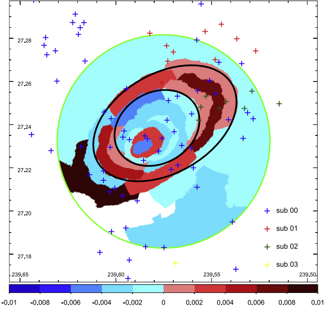
Figure 10. Redshift map of A2142. The color bar indicates the redshift difference with respect to the average X-ray redshift z_X = 0.0889 \pm 0.0009 . The black ellipses roughly mark the elliptical annulus with redshift larger than the surroundings.
