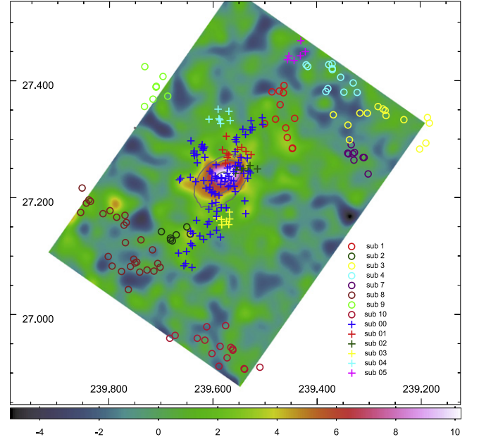
Figure 12. Weak-lensing mass map superimposed with the substructures identified with the \sigma -plateau algorithm. The color code shows the weak-lensing S/N, namely the surface mass density in units of the 1\sigma reconstruction error.
