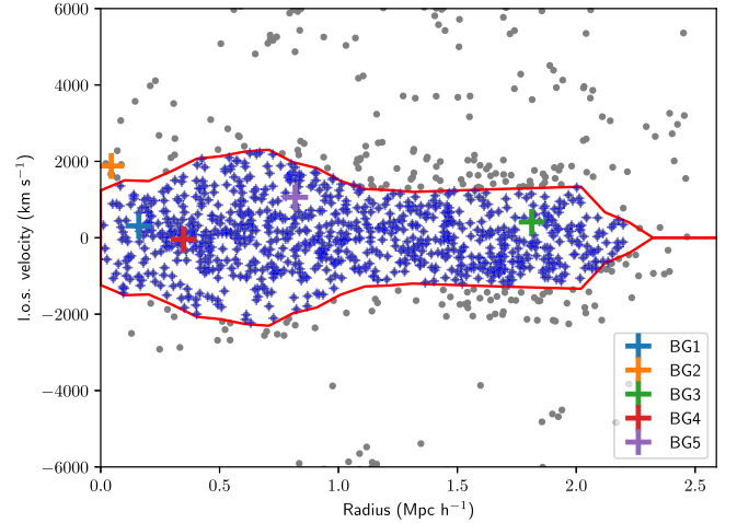
Figure 5. Redshift diagram of A2142. The solid lines show the caustic location. The blue crosses show the cluster members identified by the caustic method. We also show the location of the five brightest galaxies, BG1–5.
