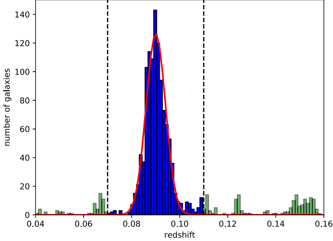
Figure 2. Redshift histogram of A2142. The green bars show the distribution of the field galaxies. The blue bars show the galaxies whose redshifts range from 0.07 to 0.11 (vertical dashed lines). The red solid line is the Gaussian fit result after the 3\sigma clipping (Yahil & Vidal 1977).
