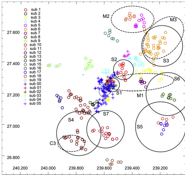
Figure 13. Substructures identified with the \sigma -plateau algorithm and with other methods in the literature. S1–S7, shown as black circles, represent the locations and sizes of the substructures identified with the \kappa -test by Owers et al. (2011). The dashed ellipses show the approximate locations and sizes of the structures identified by Einasto et al. (2018).
