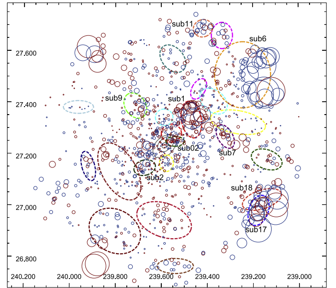
Figure 8. Results of the DS analysis based on the 1067 member galaxies identified by the 3\sigma clipping procedure on galaxy velocities. The blue and red circles represent galaxies with velocities smaller and larger than the cluster mean velocity, respectively. The radius of each circle is proportional to e^{\delta_i} . The ellipses mark the substructures identified with the \sigma -plateau algorithm. The colors of these substructures are the same as in Figures 6 and 7. We only label the names of the substructure ellipses that overlap with a clump of DS circles. The gray contour levels in the center show the distribution of the X-ray emission.
