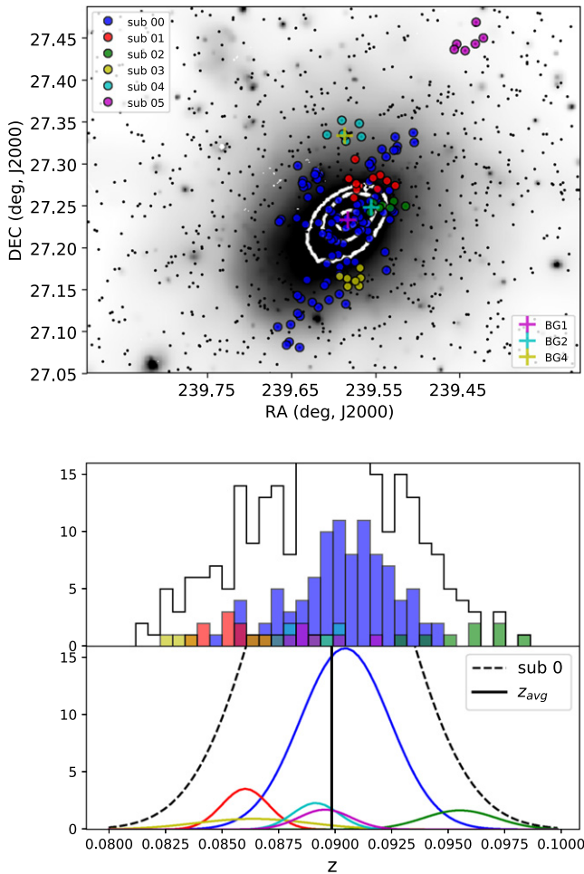
Figure 7. Same as Figure 6, but for the A2142 substructures identified with the third threshold.
