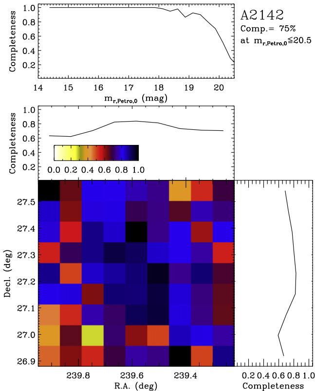
Figure 1. Spectroscopic completeness in the field of A2142.
