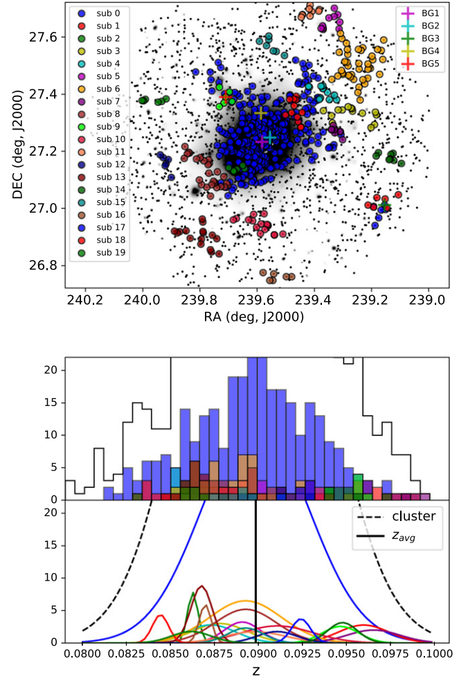
Figure 6. The upper panel shows the distribution on the sky of the A2142 substructures identified with the second threshold. The white contours and grayscale of the background image show the X-ray surface brightness from the combined X-ray observations of XMM (Tchernin et al. 2016). The middle and bottom panels show the velocity histograms of the substructures and their best Gaussian fits. The black vertical line shows the position of the mean redshift z_{\text{avg}} = 0.08982 \pm 0.00010 as a reference.
