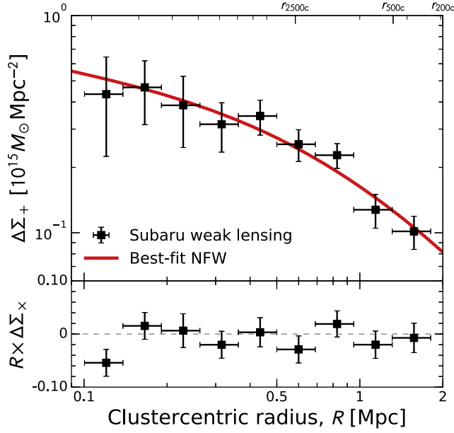
Figure 11. Tangential reduced shear profile (upper panel, black squares) of A2142 derived from our Subaru /Suprime-Cam weak-lensing observations, shown in units of projected mass density. The thick solid (red) line corresponds to the best-fit NFW profile. The lower panel shows the 45^\circ rotated \times component, which is consistent with a null signal within 2\sigma at all cluster radii.
