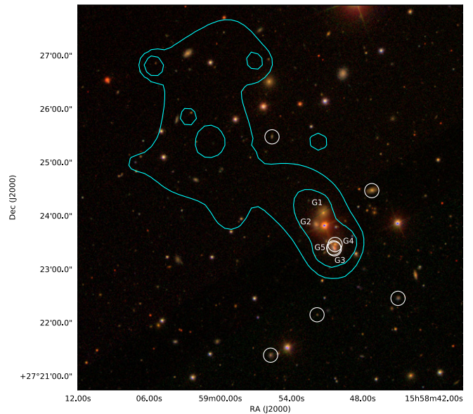
Figure 14. Zoomed-in image of the substructure sub9. The SDSS RGB image converted from the i,r,g bands is superimposed with the X-ray contours of the gas; the white circles are the members of sub9 according to the \sigma -plateau algorithm. The five galaxies in the image are labeled G1–G5, as in Eckert et al. (2017). G3 and G4 are confirmed to be members of sub9.
