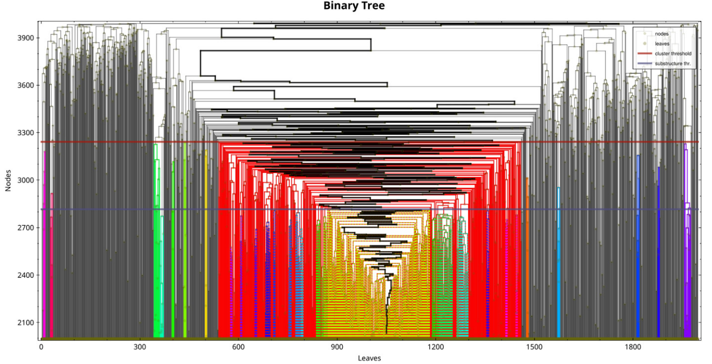
Figure 3. Dendrogram tree of 1997 redshifts in the range [0.01, 1.0] . The two solid horizontal lines are the first and second thresholds. The colors indicate different structures. The red part corresponds to sub0 in Table 2. The heavy black line shows the main branch of the binary tree.
