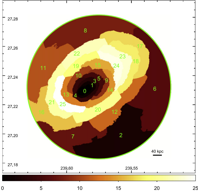
Figure 9. Region map produced on the basis of the surface brightness contours. The color bar denotes the serial number of the regions and has no physical meaning.
