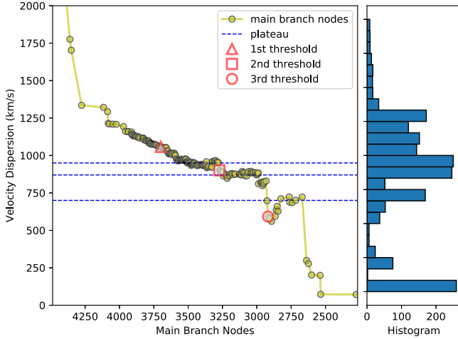
Figure 4. Velocity dispersion of the leaves of each node along the main branch of the binary tree of A2142. The histogram in the right panel shows the node numbers in different velocity dispersion bins. The blue dashed lines indicate the \sigma plateaus. The red symbols are the selected thresholds.
