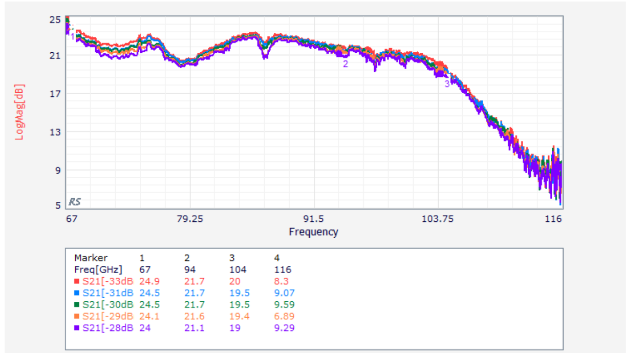
Figure 19 IL calculated when the input level is changed from -33 dBm to -28 dBm
