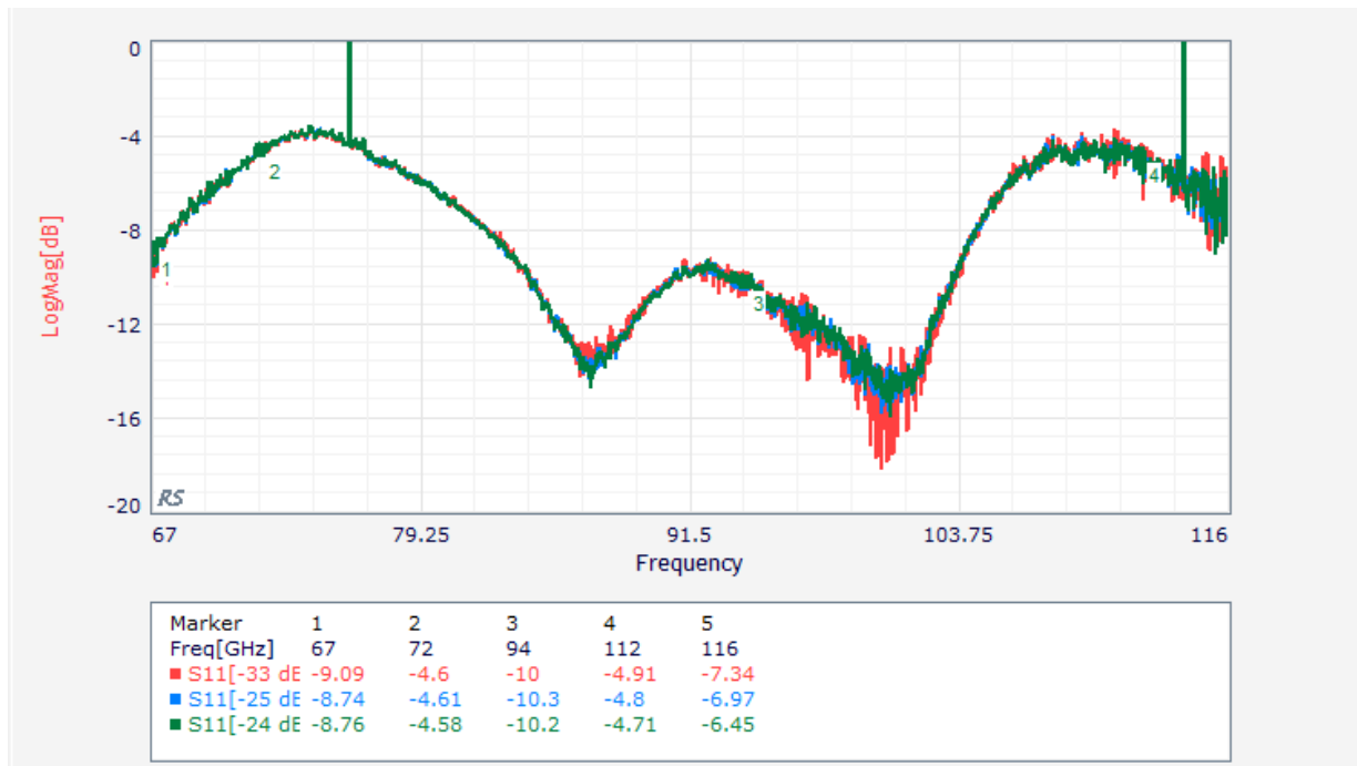
Figure 12 RL calculated when the input level is changed from -33 dBm to -24 dBm.
