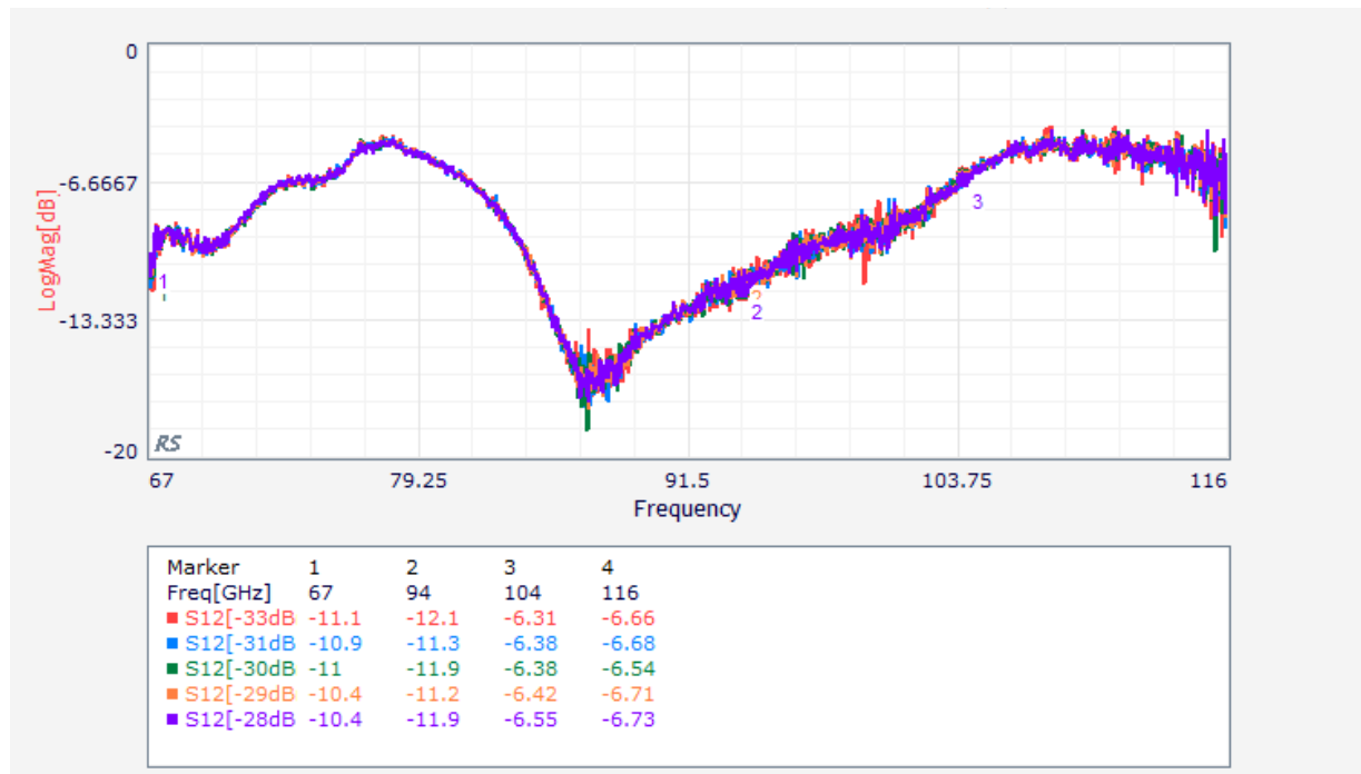
Figure 18 RL calculated when the input level is changed from -33 dBm to -28 dBm
