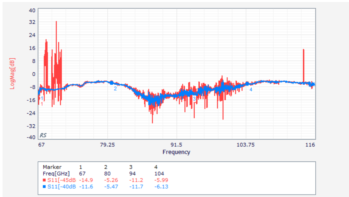
Figure 42 RL: S220 has nominal bias ; VNA input level is decreased from -45 dBm to -40 dBm.
