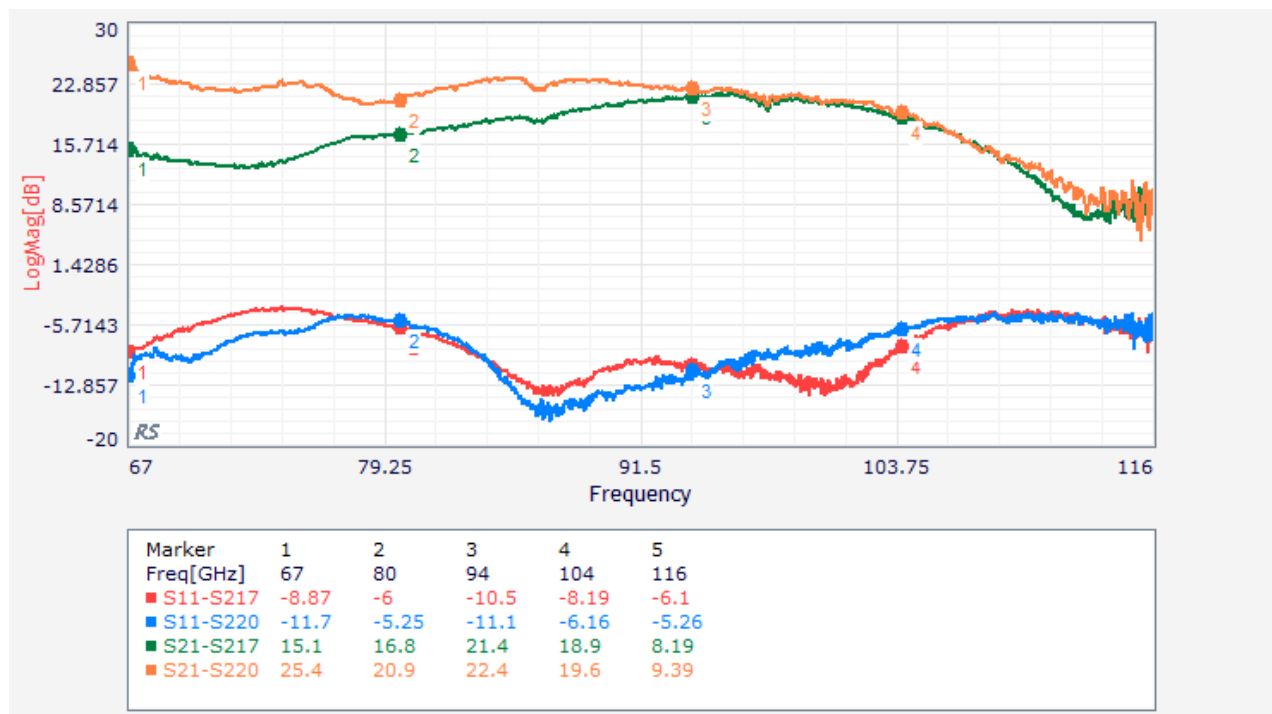
Figure 20 S11 and S21 comparison between LNAs S217 and S220.
