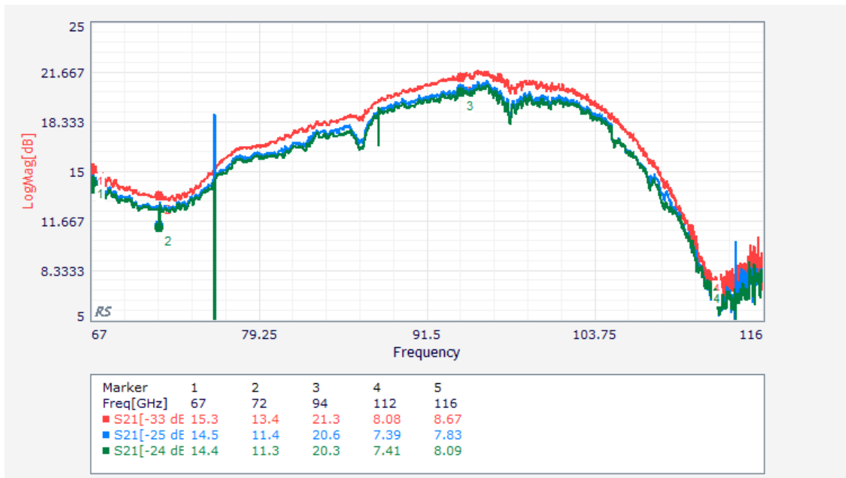
Figure 14 Gain calculated when the input level is changed from -33 dBm to -24 dBm
