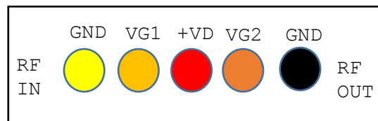
Figure 3 electric connection scheme
