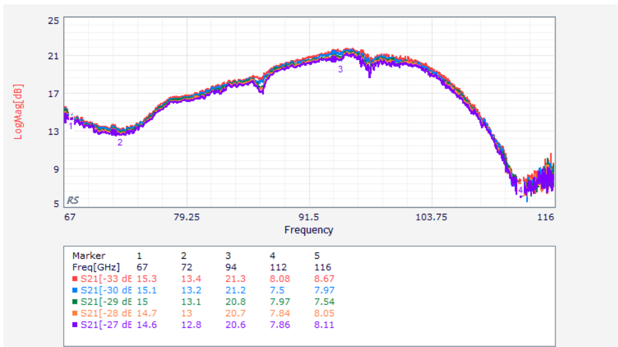
Figure 13 gain calculated when the input level is changed from -33 dBm to -27 dBm.
