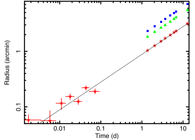
Figure 7. Left-hand panel: angular size of the inner ring as a function of time; each point (red) was obtained by fitting with a constant plus a Lorentzian model the radial profile obtained in consecutive bin times (with a varying length) starting from the burst; the solid line is the best fit \theta(t) = (0.884 \pm 0.045) \times t^{0.5} . Right-hand panel: joint fit with the points taken from Tiengo et al. (2010). The red stars, green triangles and blue squares indicate the angular radii of the three rings caused by the burst on January 22. Error bars are at 1\sigma in both figures.
