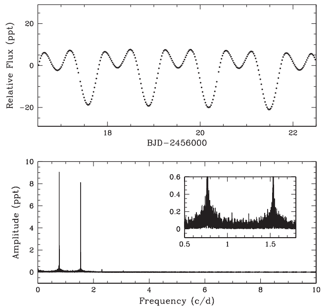
Figure 5. Upper panel: portion of the LC of KIC 7599132 observed by Kepler . Bottom panel: periodogram in the interval 0–10 c/d based on the Q0–Q17 data. The insert show the periodogram around the main frequency and the first harmonic (see the text).
