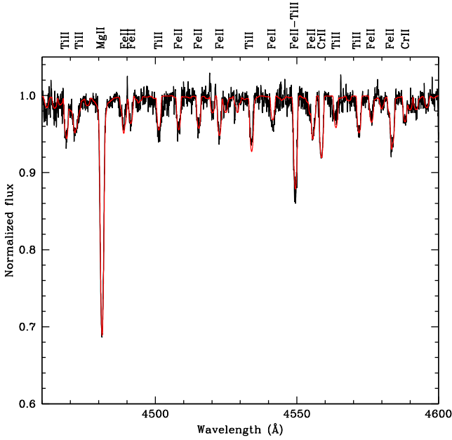
Figure 3. Portion of spectrum for KIC 7599132 with overimposed (red lines) the synthetic spectrum computed with the parameters derived in this study. The chemical abundances for the identified spectral lines are solar.
