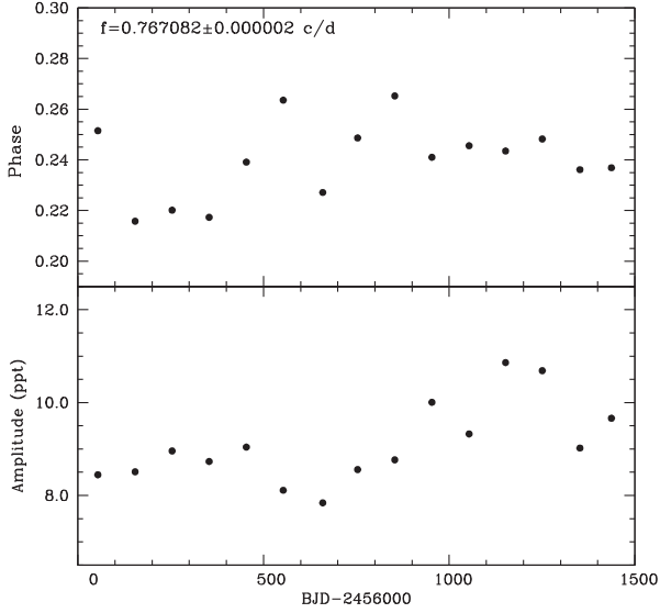
Figure 6. Phase (top panel) and amplitude (bottom panel) variation for the main frequency f = 0.767082 \pm 0.000002 c/d KIC 7599132. Filled circles represents the main frequency computed for a chunk of data of 100 d (with the exception of the last one). The sizes of the symbols are approximately of the order of the errors.
