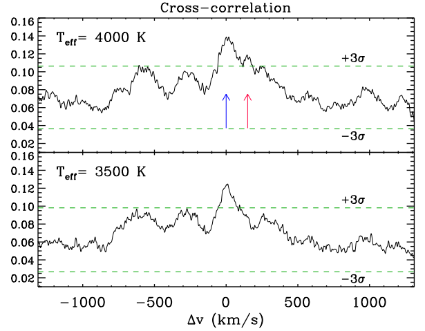
Figure 9. CCFs between simulated composite spectra and RV templates. The spectra of the two components (synthetic ATLAS9 spectra) have been shifted by 150 \text{ km s}^{-1} and weighted according to the parameters quoted in Table 2. In the upper panel, an effective temperature of 4000 K has been adopted for the secondary component, while in the bottom, it has been fixed to 3500 K. The two vertical arrows mark the RV of the components and the dashed lines delimit the \pm 3\sigma confidence region.
