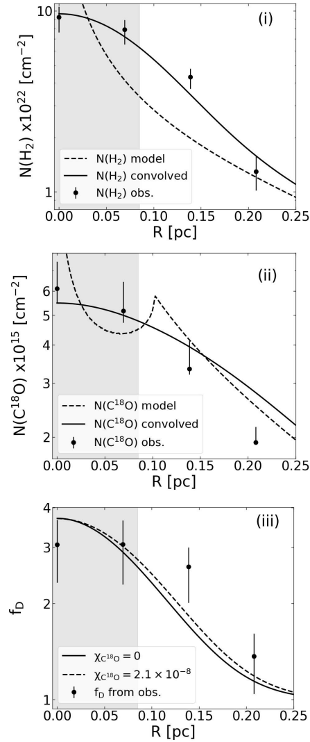
Fig. 3. Column densities N(\text{H}_2) and N(\text{C}^{18}\text{O}) are plotted in panel (i) and (ii), respectively, as a function of the projected distance from the centre ( R ) of clump-5. In panel (iii) we show the mean f_D profile in C5. Dashed-profiles show: the 1.o.s.-integrated profiles of eq. 3 (panel i) and same for N(\text{C}^{18}\text{O}) assuming f_D = 10 for R < R_{dep} (panel ii), while the R_{dep} position corresponds to the cusp; solid-drawn curves are the profiles convolved with the Herschel beam at 500\ \mu\text{m} (FWHM: grey-shaded area). Dashed- and solid-profiles in panel (iii), show the modeled f_D profiles. Black points are the observed values. The plots are adapted from Sabatini et al. (2019) and reprinted with permission.
