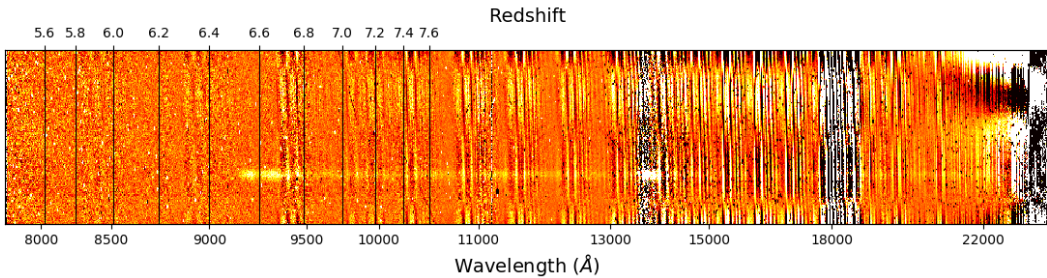
Figure 16. Two-dimensional spectrum of PSO J344.1442–02.7664 obtained with Magellan/FIRE. A strong \text{Ly}\alpha break is clearly seen around the observed-frame wavelength of 9100 \text{ \AA} which means that the \text{Ly}\alpha emission is redshifted to z \sim 6.5 .
