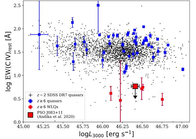
Figure 6. The CIV rest-frame EW as a function of continuum luminosity at 3000 \text{ Å} . The black dots show sample of z \sim 2 quasars from Shen et al. (2011). The z > 5.7 normal quasars (blue squares) and WLQs (red squares) which are taken from Shen et al. (2019) are also shown. It is clear that PSO J083+11 is the 3\sigma outlier at the low-end of normal quasars' \text{EW}(\text{CIV})_{\text{rest}} log-normal distribution.
