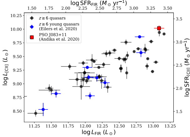
Figure 13. The comparison between the star formation rate estimated from the dust continuum luminosity (following Murphy et al. 2011 and Kennicutt & Evans 2012) and the [\text{C II}] luminosity (following De Looze et al. 2014) using assumption of T_{\text{dust}} = 47 \text{ K} . A sample of z \gtrsim 6 quasars from literature (black dots, see text) and z \gtrsim 6 young quasars (blue dots, Eilers et al. 2020) are shown. PSO J083+11 (red square) shows values of L_{[\text{C II}]} and L_{\text{FIR}} comparable to those high- z quasars with the highest SFR and FIR emission. For clarity, the error bars of PSO J083+11 have been multiplied by three.
