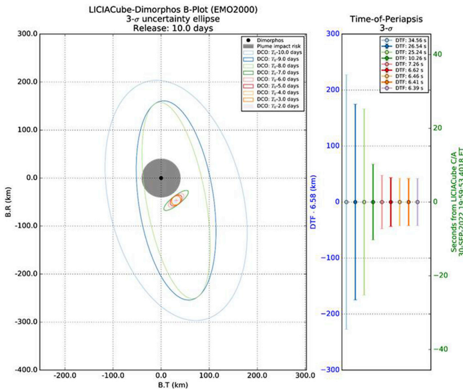
Fig. 4. LICIAcube position uncertainty (3-sigma) at C/A in the Dimorphos-relative B-plane. The uncertainty is reported as an in-plane contribution provided by an ellipse centered in the probe nominal position and an extension expressed by 3 parameters: semi-major axis, semi-minor axis, and a rotation angle. The out-of-plane contribution is given as the Differential Time of Flight (DTF), which represents the uncertainty about the epoch of the flyby to occur. This time uncertainty was converted as an approximated distance by multiplying for the LICIAcube relative speed of 6.58 km/s.
