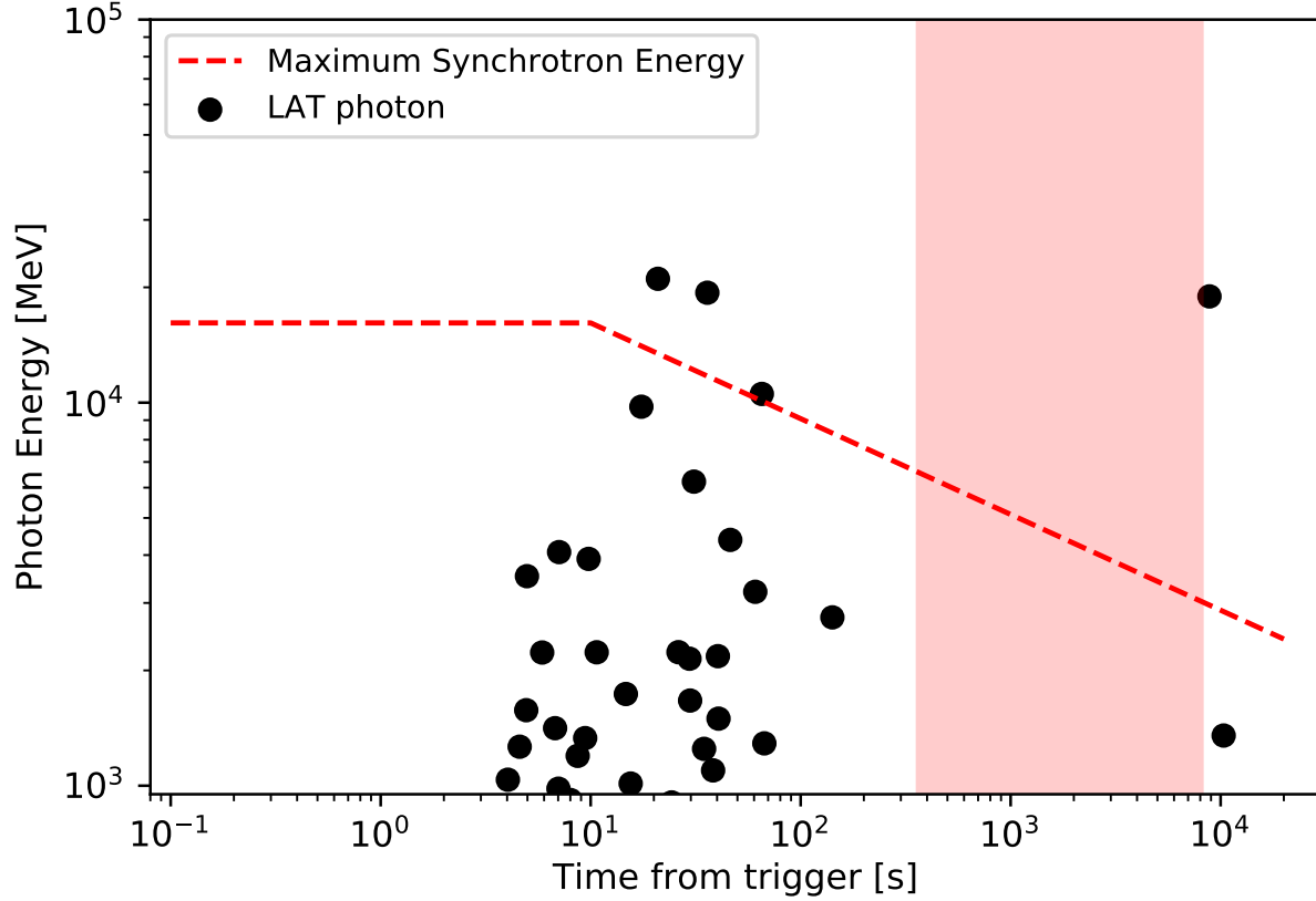
Figure 9. Photon energy versus time. Photons with energies > 1 GeV and > 90\% probability of association with GRB190114C are indicated with black dots. Dashed line represents the maximum synchrotron limit for the adiabatic jet with the wind case. Here we use the estimated bulk Lorentz factor \Gamma_{\text{bulk}} = 213 , E_{\text{iso}} = 3.5 \times 10^{53} erg and the efficiency of total shock energy in converting into the gamma-ray emission \eta = 0.2 . The deceleration time for the wind case is calculated with A_{\star} = 0.2 . The red shaded region represents a non-observable period for GRB 190114C due to Earth occultation.
