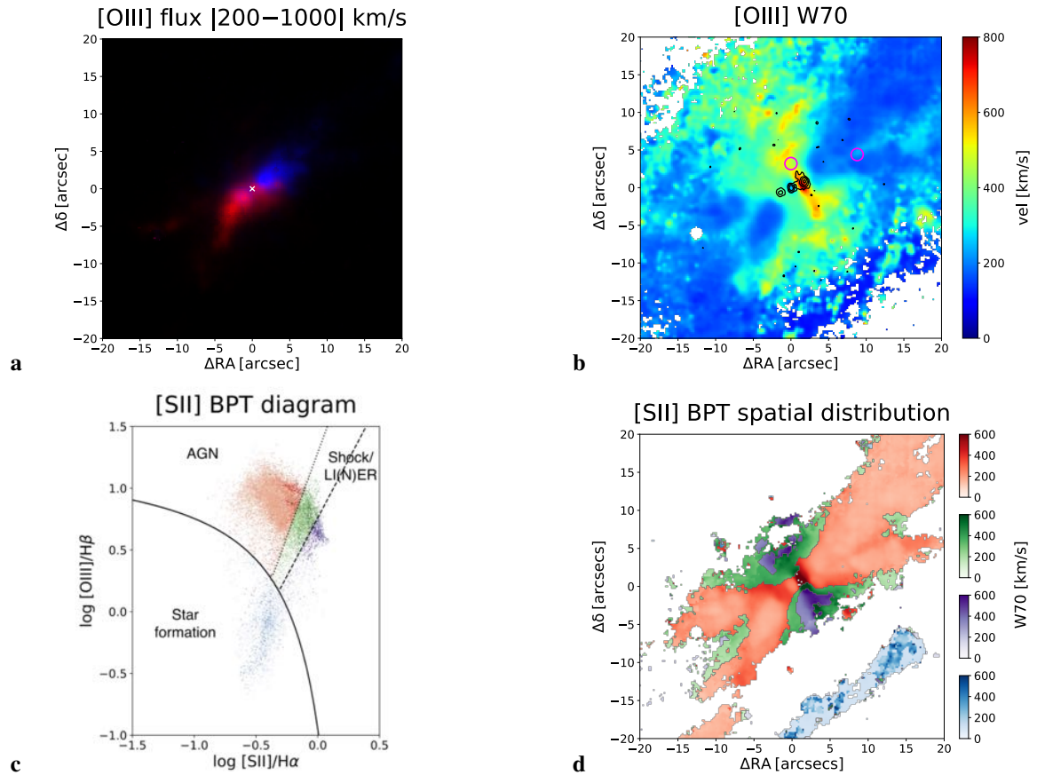
Fig. 2. IC 5063. (a) [O III] flux integrated from the fitted profile in the velocity range \pm[200 – 1000] km s ^{-1} (blue when negative, i.e. approaching, red when positive, i.e. receding) with respect to the stellar velocity in each pixel (to avoid including the contribution to the flux from the gas that rotates in the disc). It shows the bulk of the high-velocity outflow. (b) [O III] W70 map, i.e. the difference between the 85th and 15th percentile velocities of the modelled line profile. The map has been re-smoothed with a Gaussian kernel having \sigma = 1 pixel for better visual clarity. The radio contours are the same as in Fig. 1c. Magenta circles indicate 4-spaxel radius extraction apertures of the spectra displayed in Fig. 3. (c) [O III] \lambda 5007/H\beta vs. [S II] \lambda\lambda 6716,6731/H\alpha BPT diagram and (d) associated spatial distribution. The colour intensity in the diagram and the map is coded according to the [O III] W70. The solid curve defines the theoretical upper bound for pure star formation (Kewley et al. 2001). The dashed line represents the Kewley et al. (2006) demarcation between Seyfert galaxies and shocks or LI(N)ERs, while the dotted line is the Sharp & Bland-Hawthorn (2010) bisector line between AGN- and shock-ionisation. SF-dominated regions are then marked in blue, AGN-dominated ionisation in red, and purple and green mark shock-ionised or LI(N)ER regions. As in Fig. 1c, the maps are zoomed in the central 40'' \times 40'' compared to the full-FOV image in Fig. 1b. An S/N cut of 3 has been applied to the maps, together with a cut on high velocity dispersions resulting from poor fits (see text for details).
