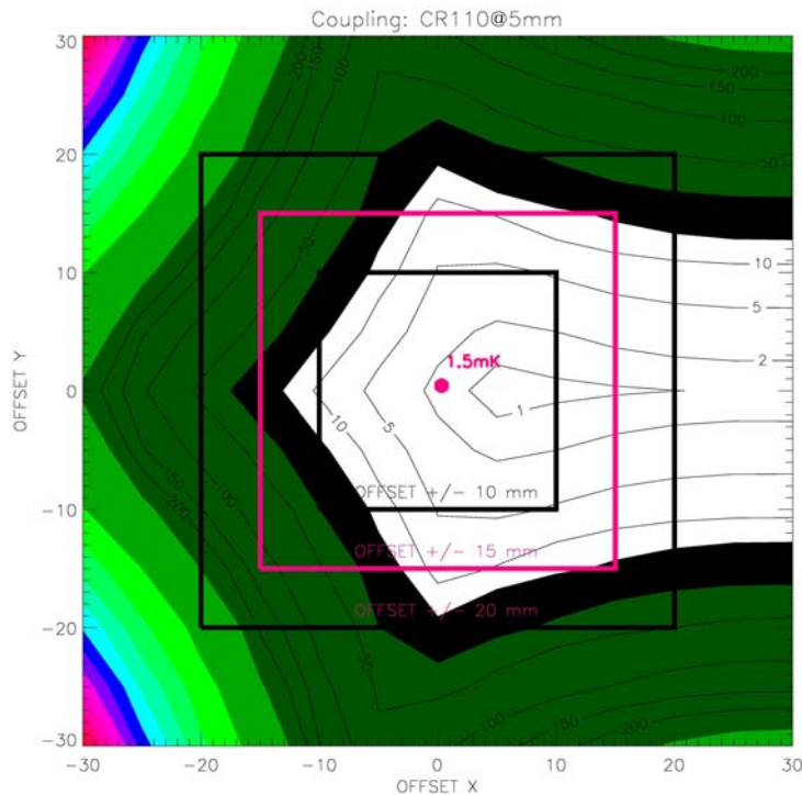
Figure 20 Maximum coupling between LFI feeds, depending on displacement (CR110 layer 5mm thick) ; values in mK; the three offset regions [ X=\pm 10 mm , Y=\pm 10 mm], [ X=\pm 15 mm , Y=\pm 15 mm], [ X=\pm 20 mm , Y=\pm 20 mm] are displayed
